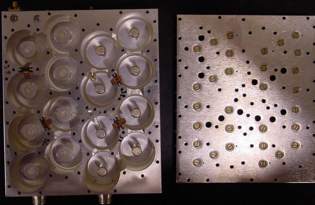
Digivance LRCS 1900 MHz Duplexer Bottom Open View - Typical
