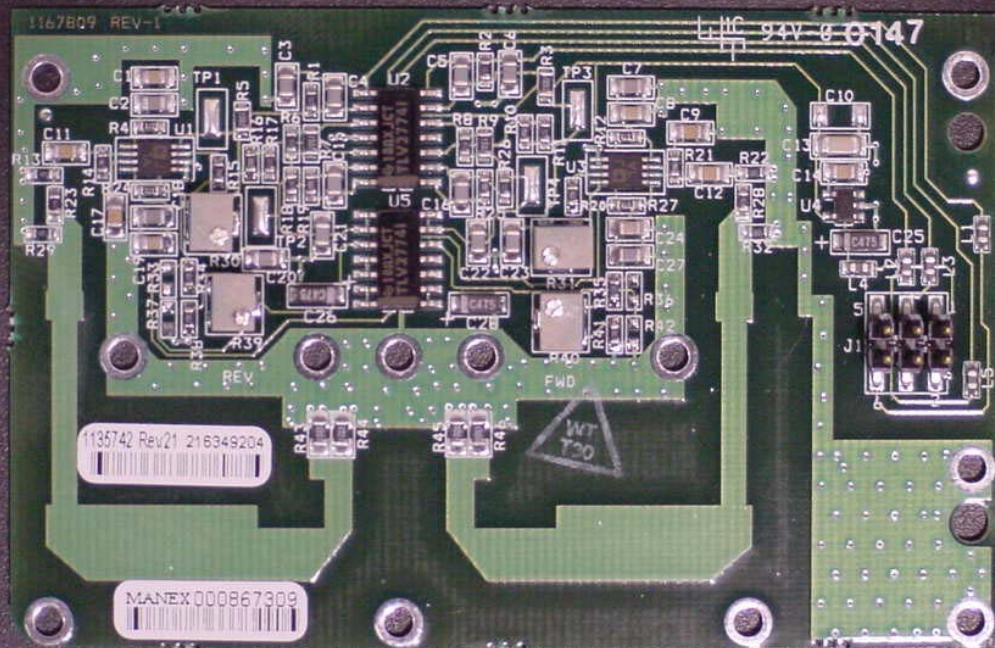
Digivance LRCS Power Monitor Board Top View
