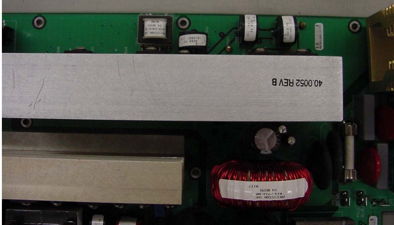
Digivance LRCS Power Supply Board Top View - Upper Right
