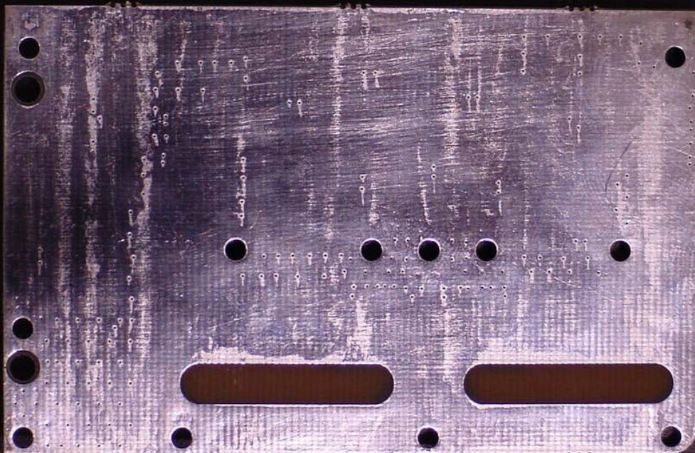
Digivance LRCS Power Monitor Board Bottom View
