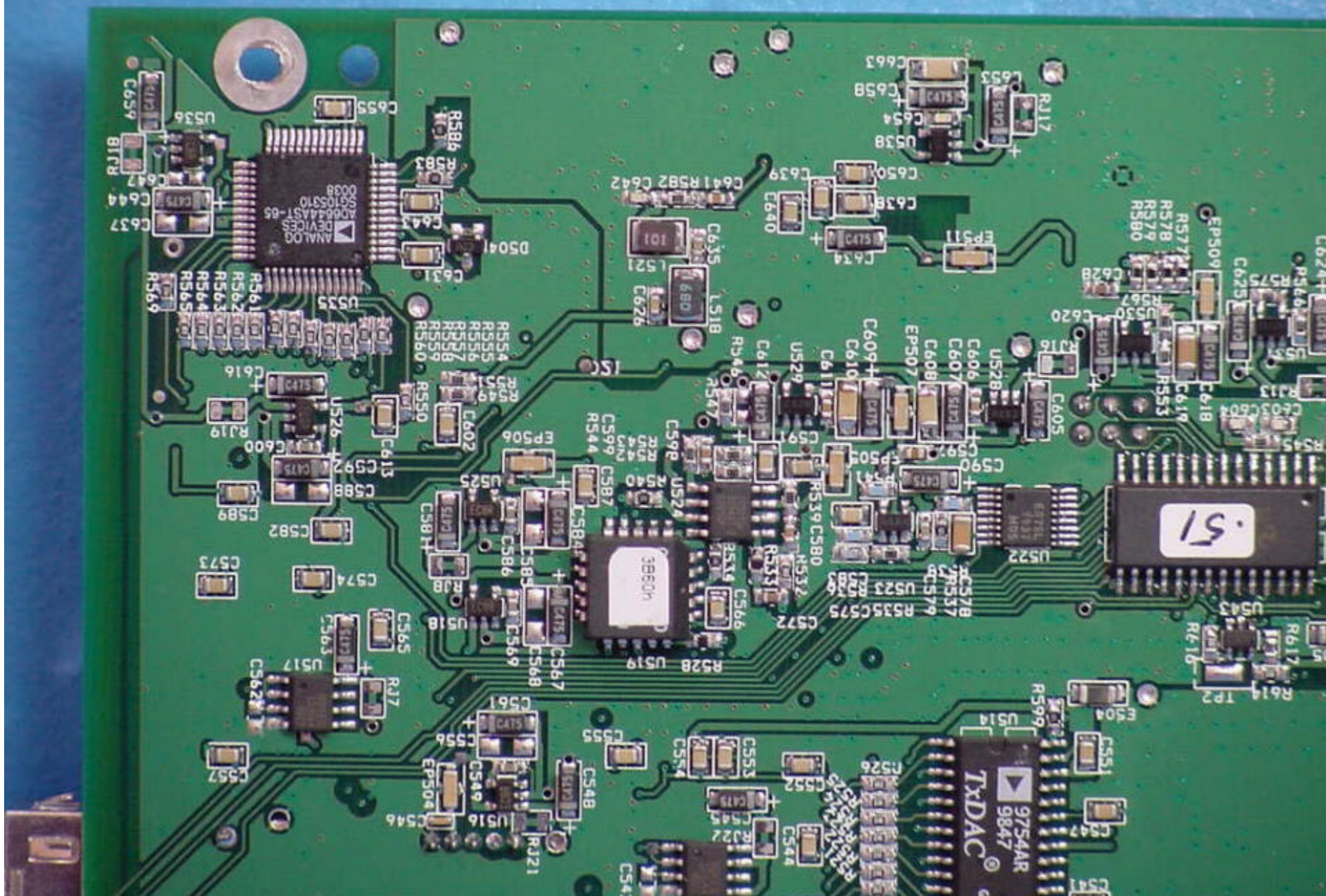
Digivance Digital Remote Unit (DRU) Back Top Left
