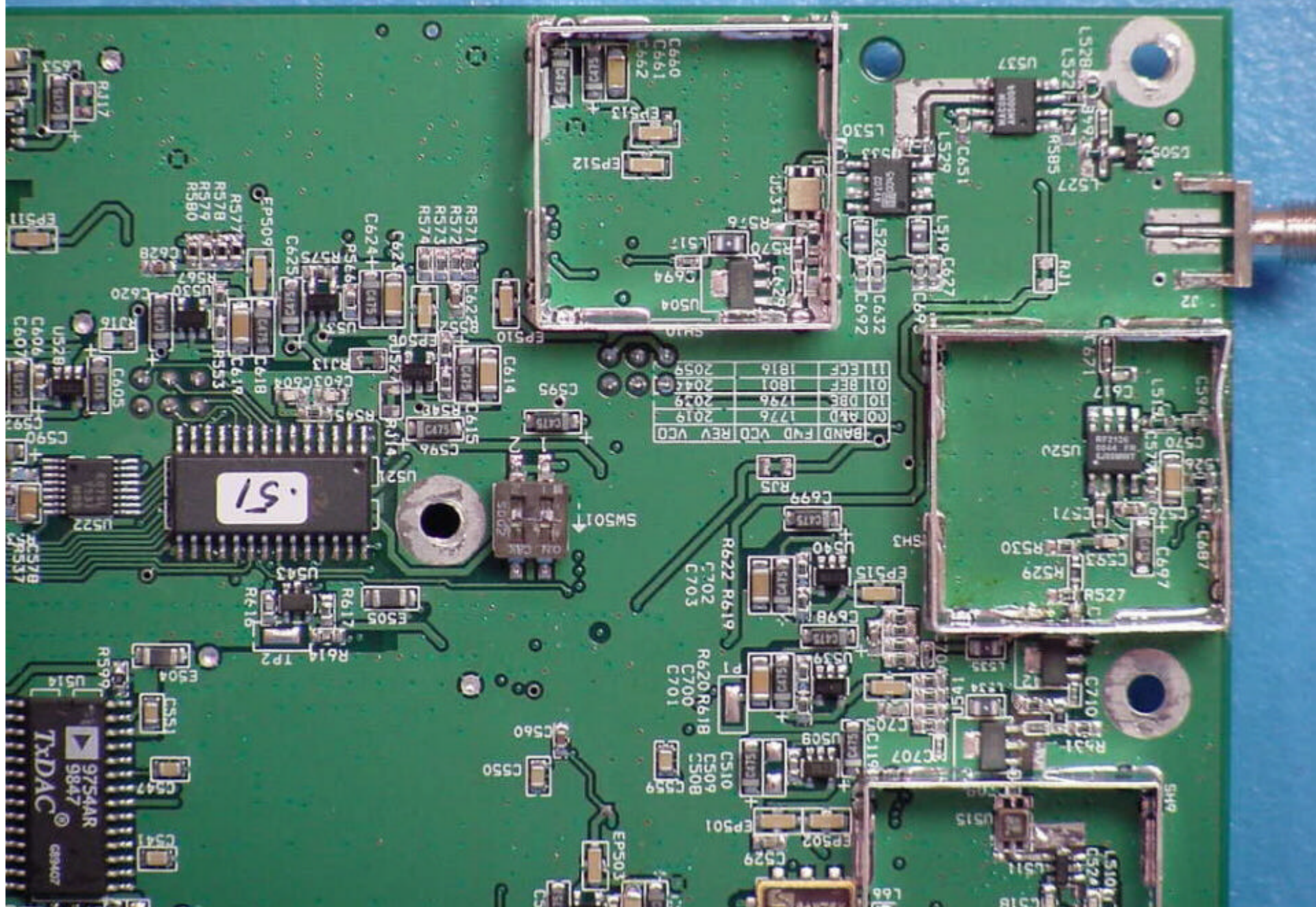
Digivance Digital Remote Unit (DRU) Back Top Right
