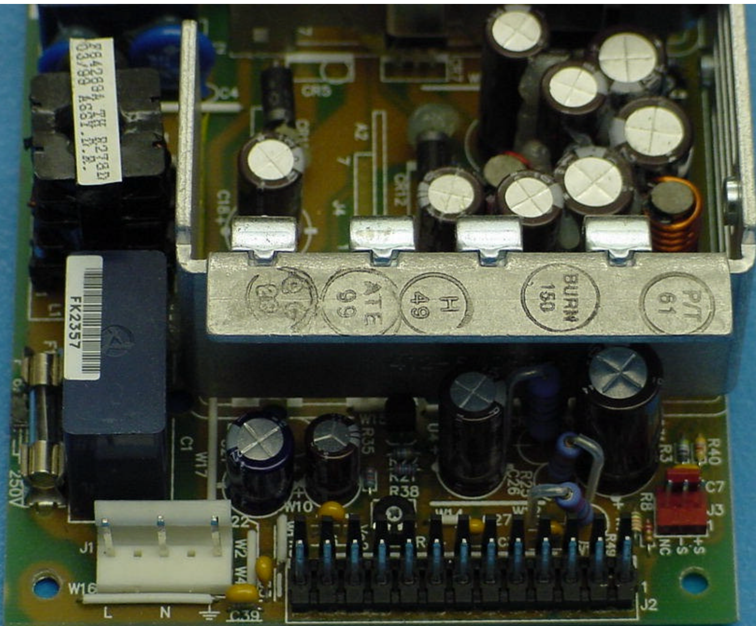
Digivance 1900 MHz Remote Interface Unit Power Supply - Detail #1 View
