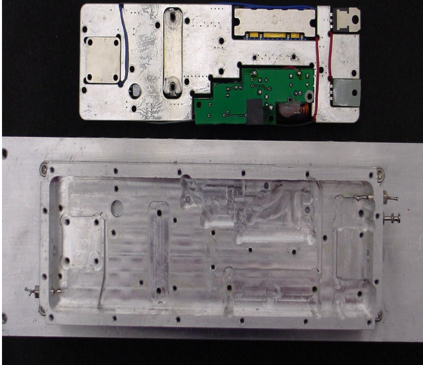
Digivance 1900 MHz Remote Interface Unit Power Amplifier - Internal Bottom View
