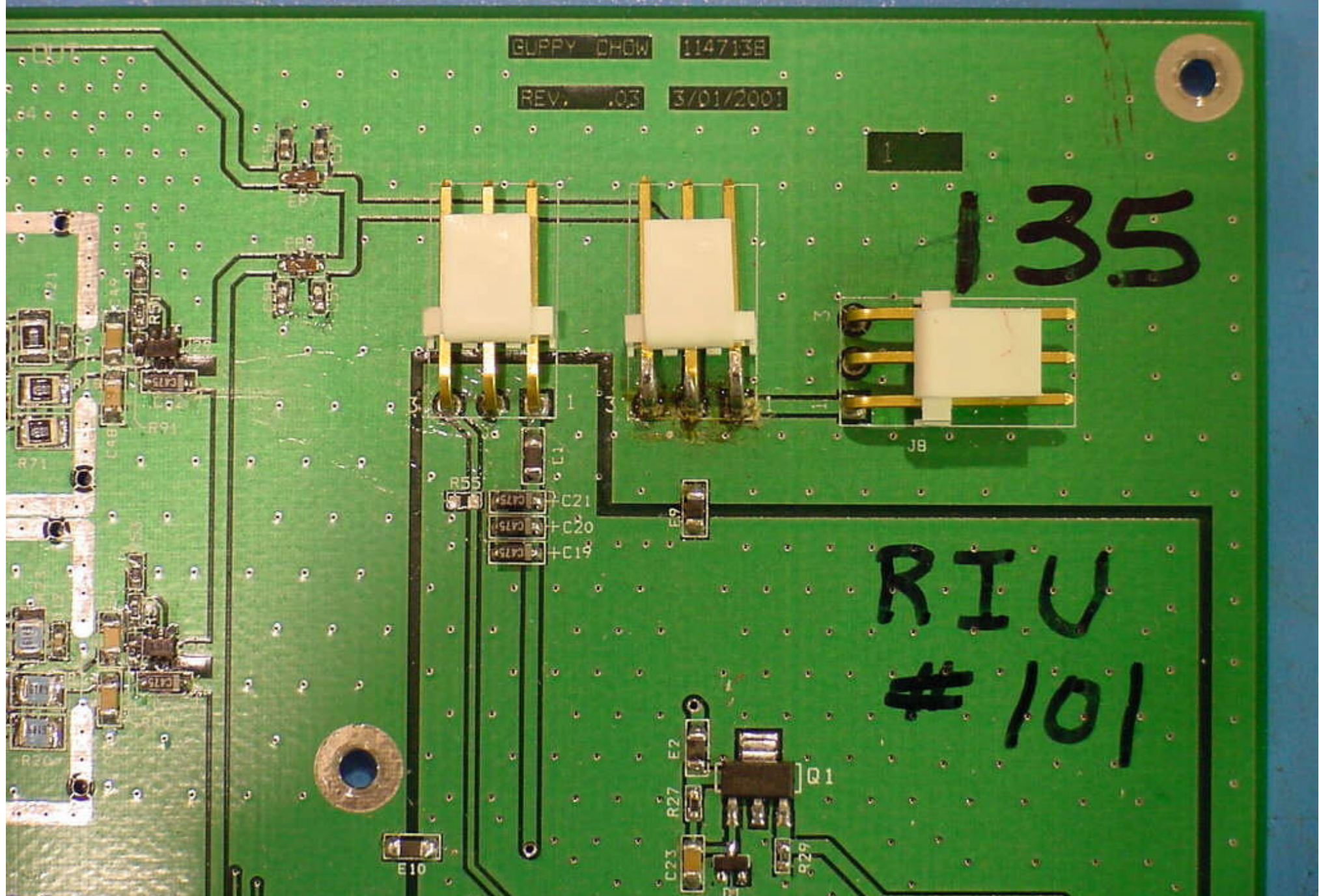
Digivance Remote Interface Unit (RIU) Control Board Top Zoom Upper Right
