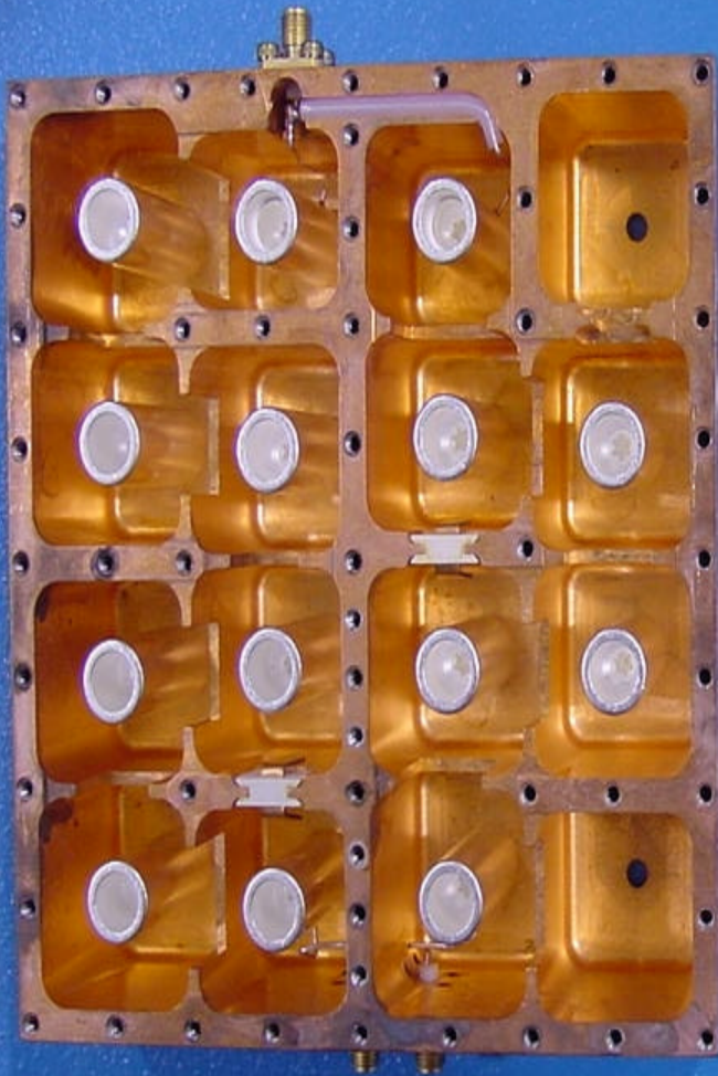
Digivance Remote Interface Unit (RIU) Model DGVI-120000RIU Duplexer (Top View)
