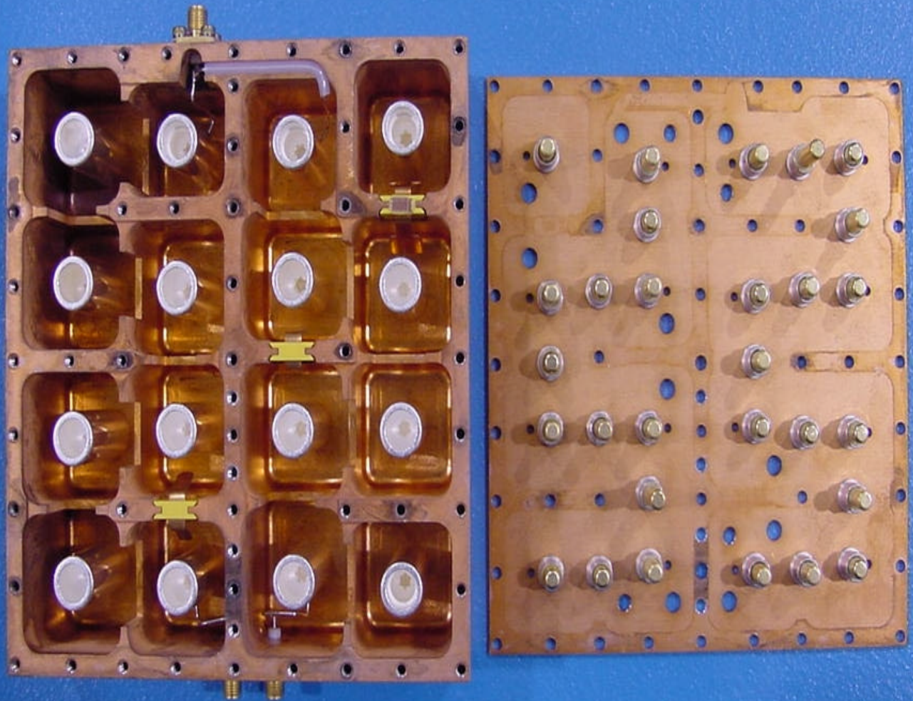
Digivance Remote Interface Unit (RIU) Model DGV1-110000RIU Duplexer (Top View)
