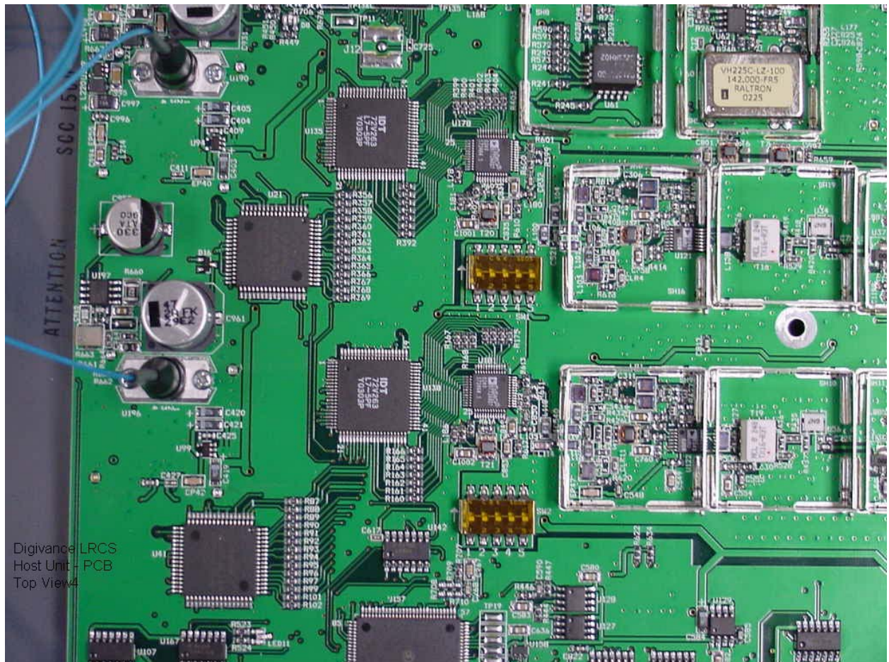
Digivance LRCS Host Unit - PCB Top View3
