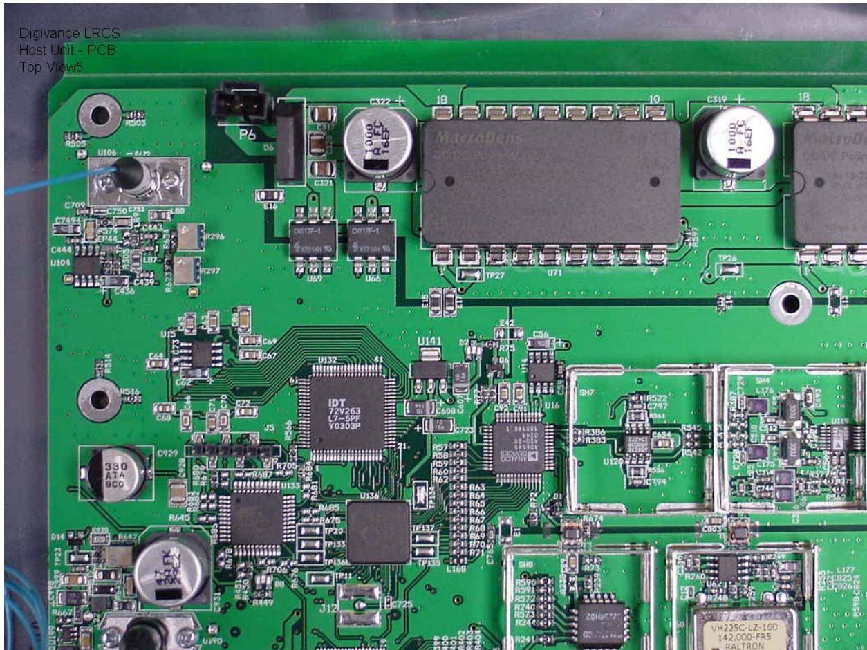
Digivance LRCS Host Unit - PCB Top View6
