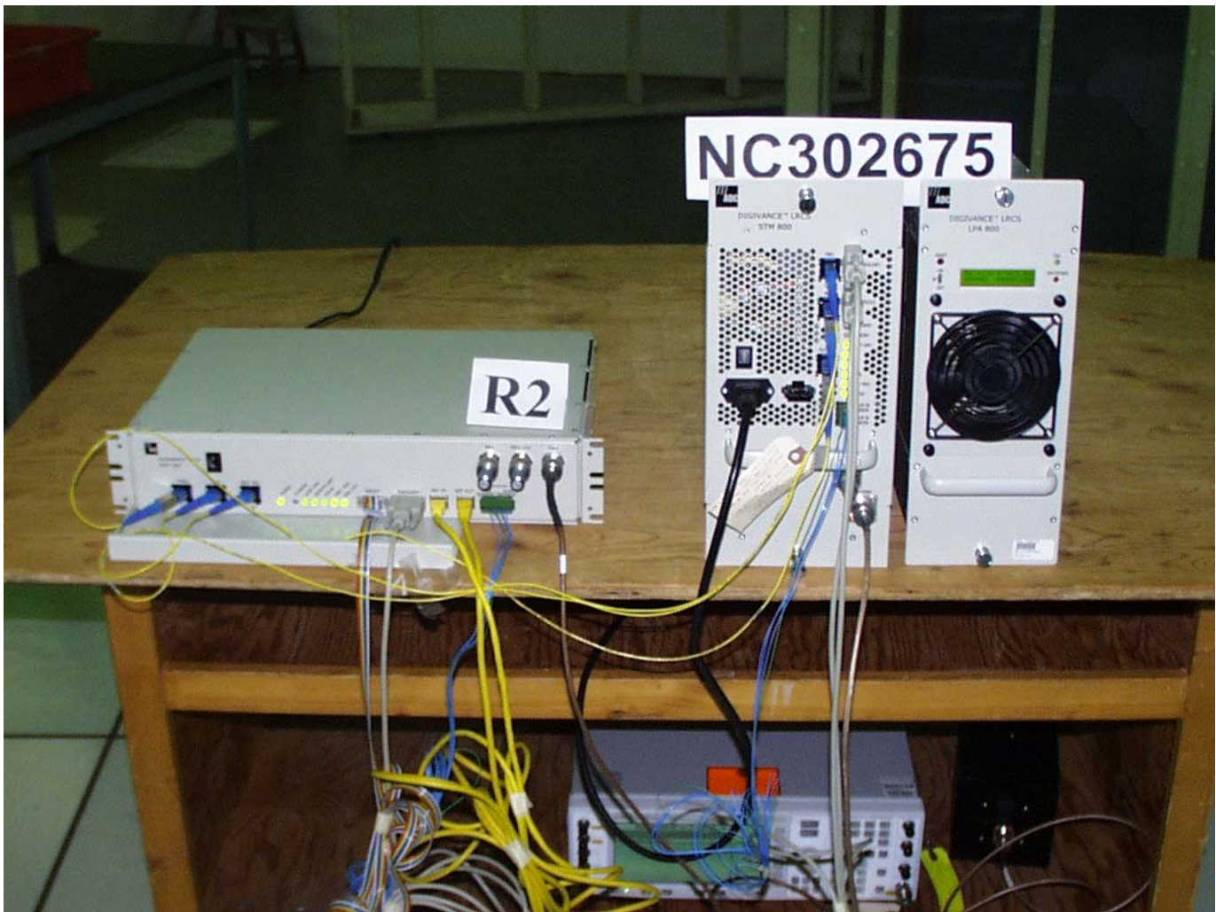
Radiated Emissions Test Setup Photo:
