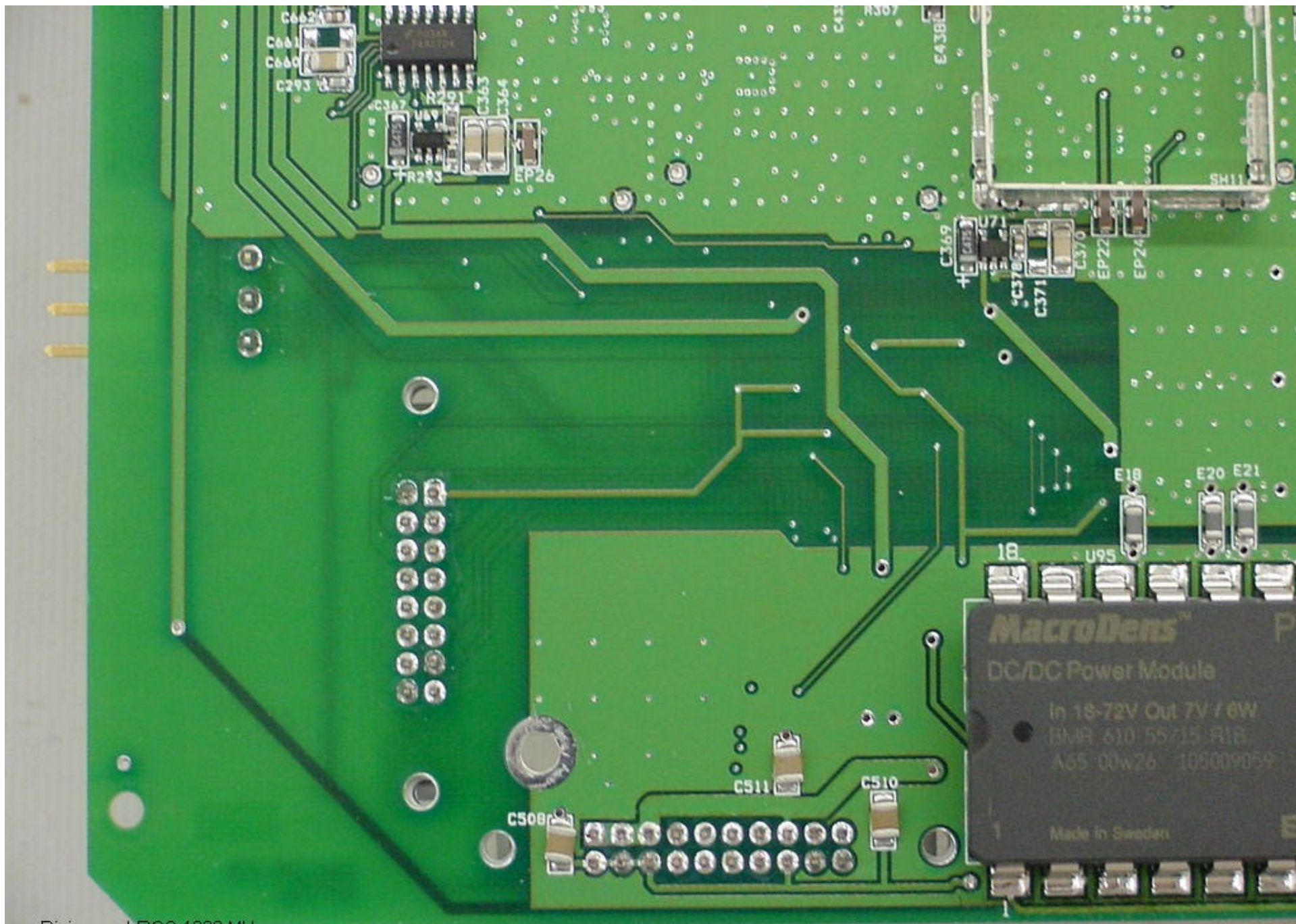
Digivance LRCS 1900 MHz Signal Transport Module Control Board - B1
