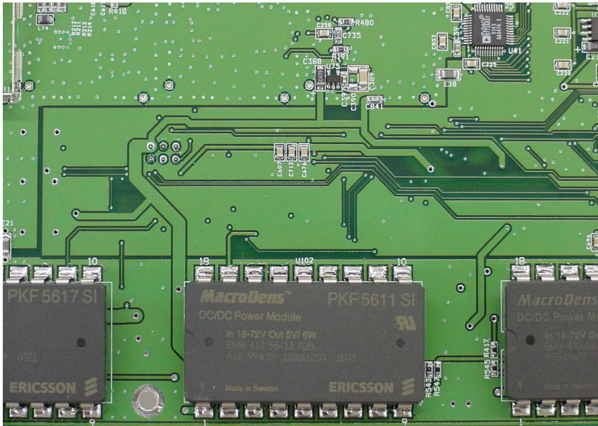
Digivance LRCS 1900 MHz Signal Transport Module Control Board - B2
