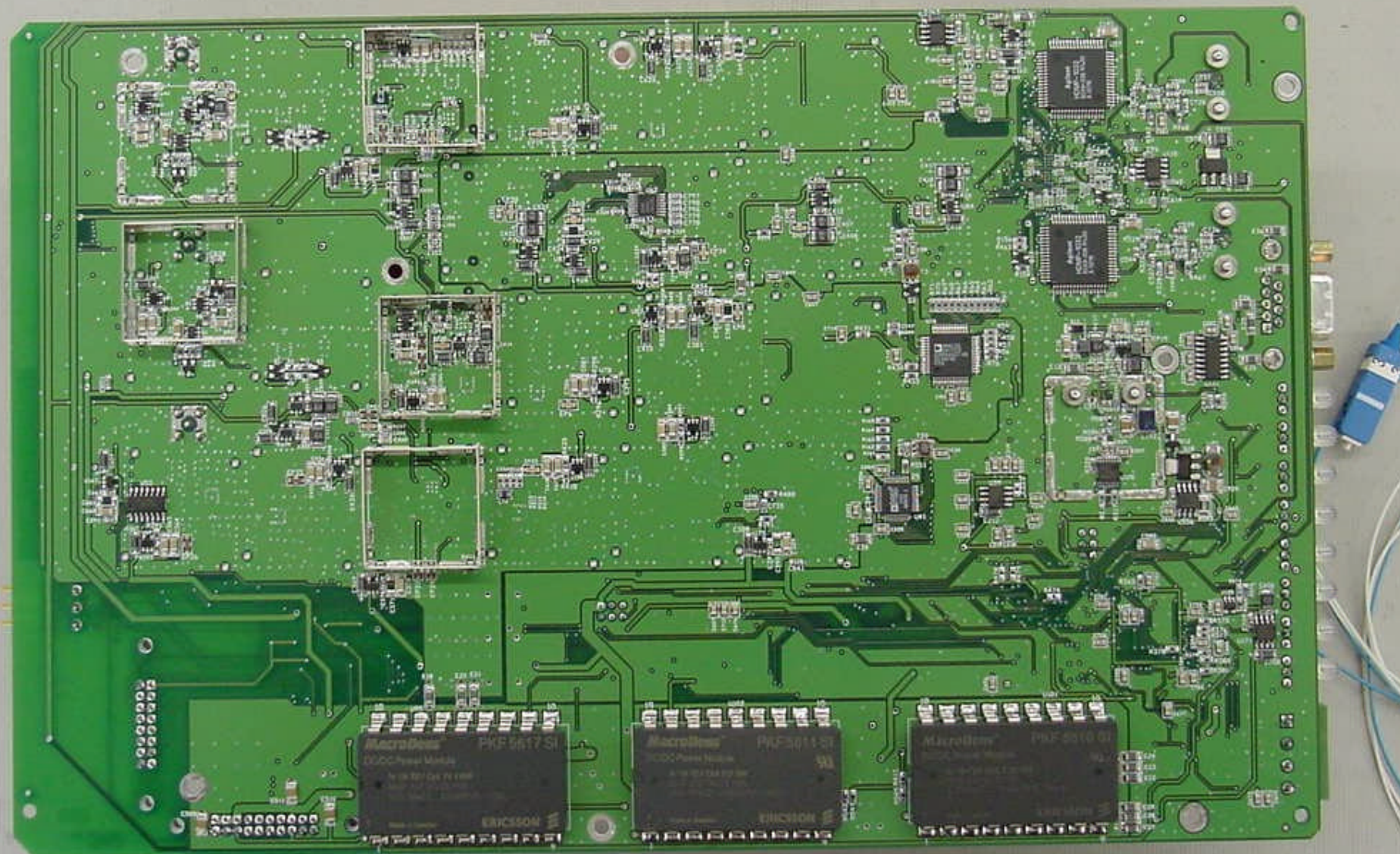
Digivance LRCS 1900 MHz Signal Transport Module Control Board Bottom View
