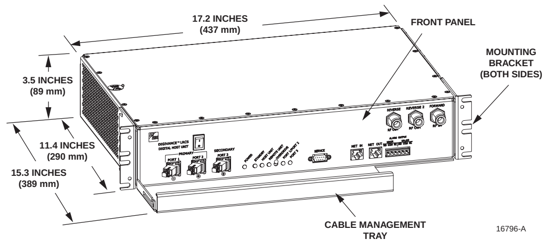
Figure 2-1. Host Unit
