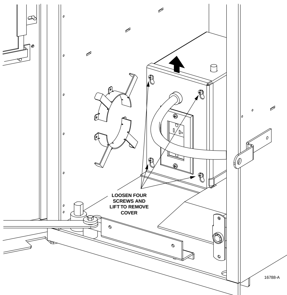
Figure 5. Accessing AC Power Wiring
