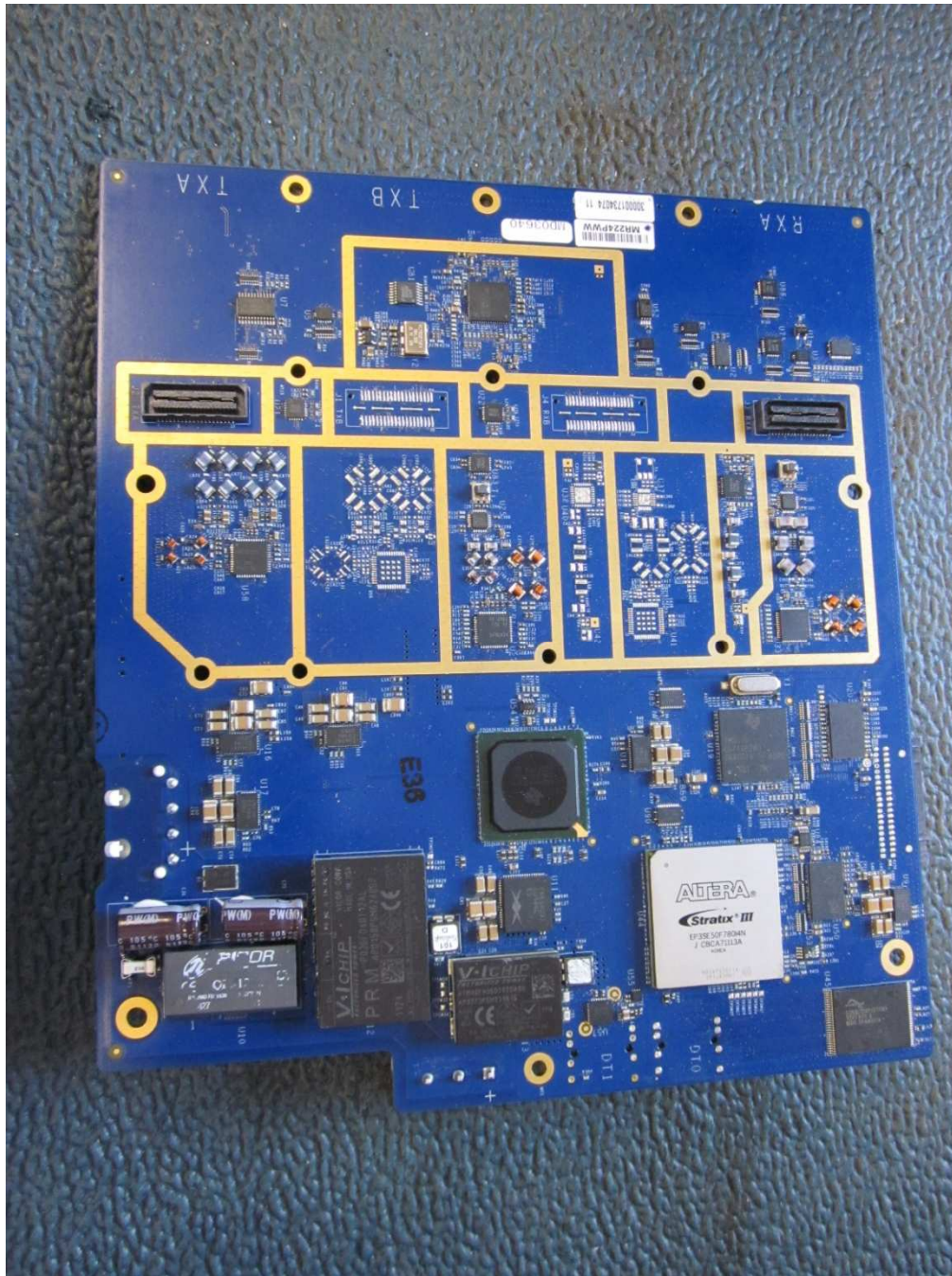
Motherboard – Front #1
