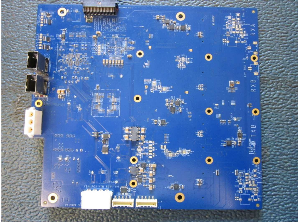
Motherboard – Back #1
