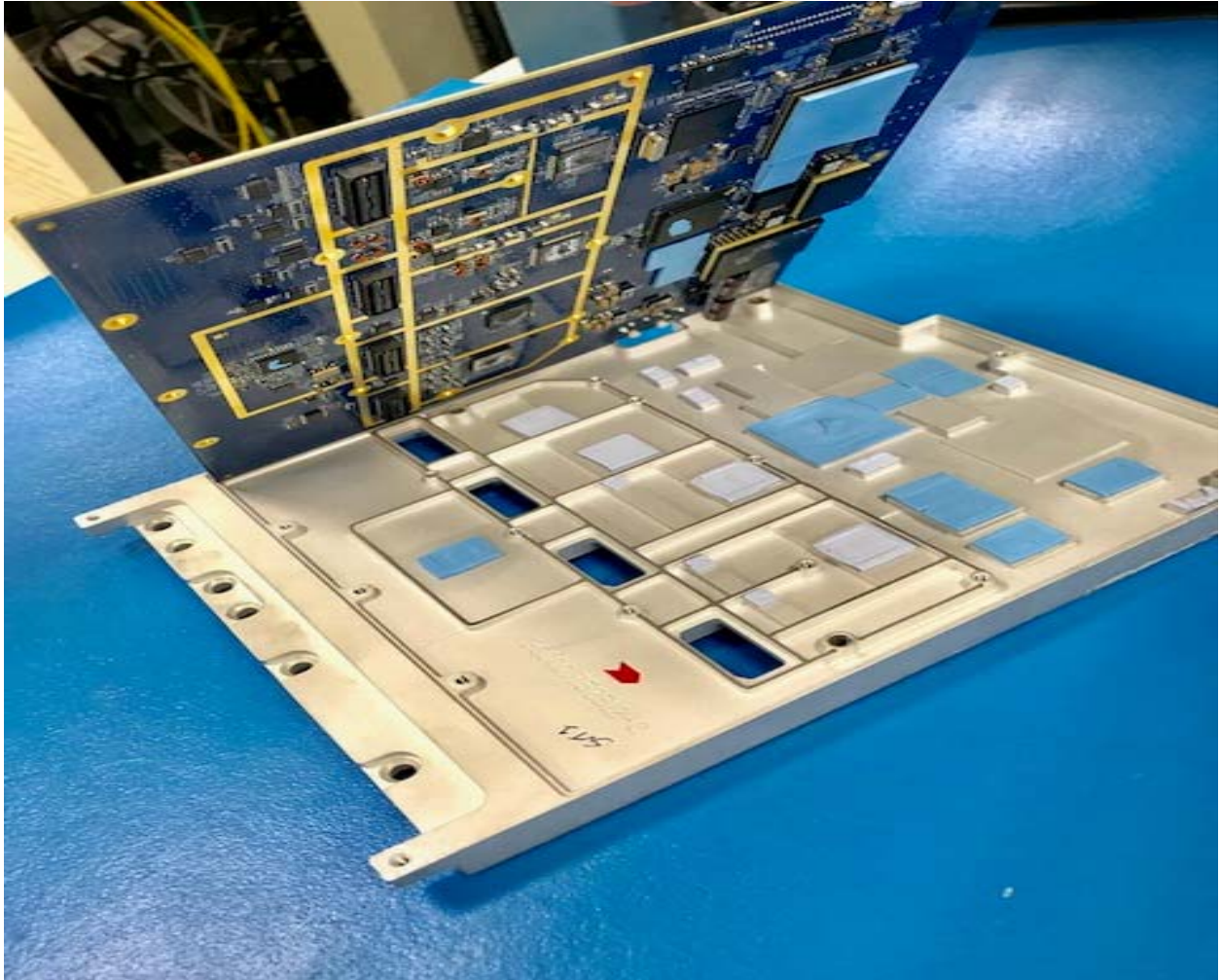
Motherboard and Carrier Plate #1
