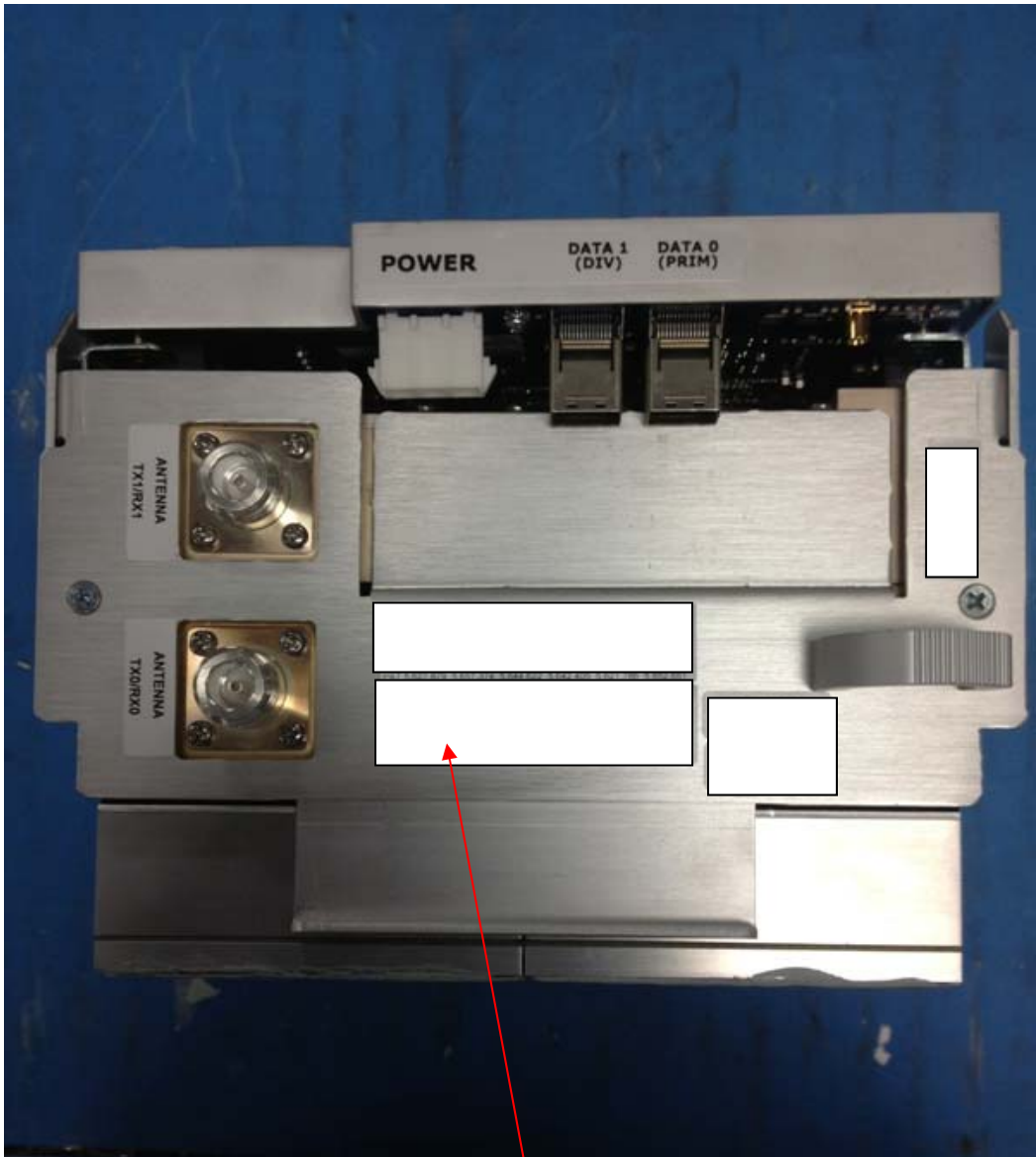
FCC/IC Label Location
