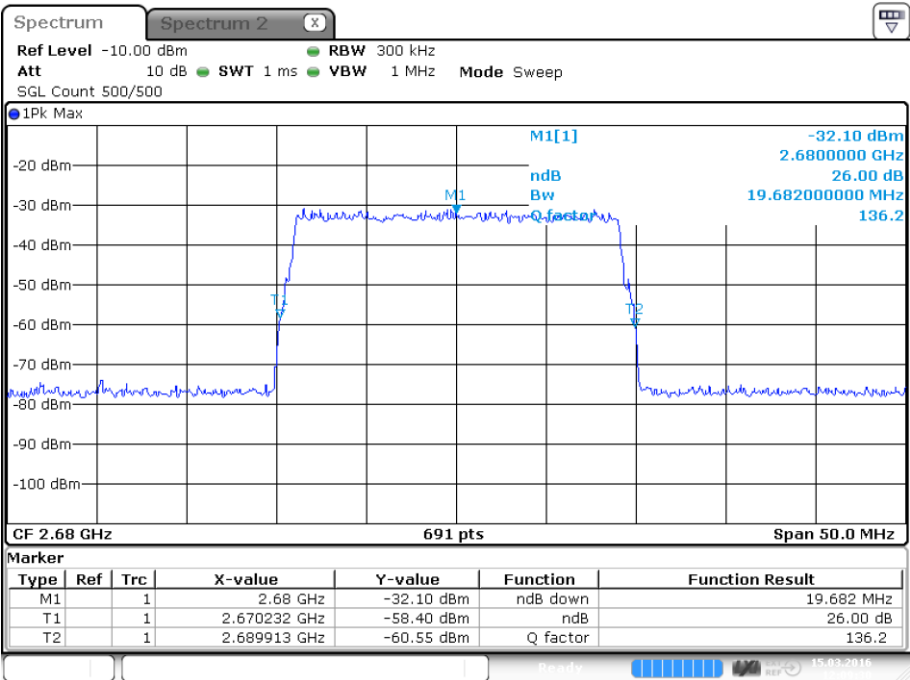
plot 6.3.2.3-#2 Occupied Bandwidth: $2.1049; Test results; 26dB Bandwidth; LTE top Input
