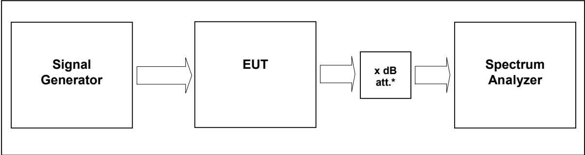
External Attenuator DL x dB = 20 dB figure 9-#1 Test setup: Frequency Stability
