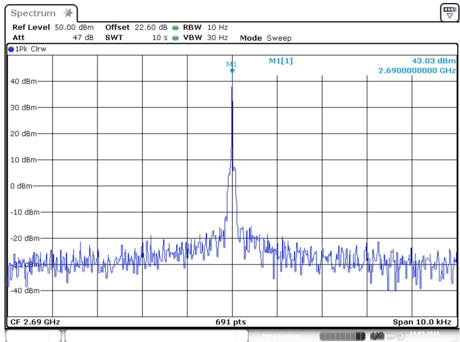
plot 9.3.1.10-#3 Frequency Stability; Test results; Downlink; @ -30 C; top; voltage 100%
