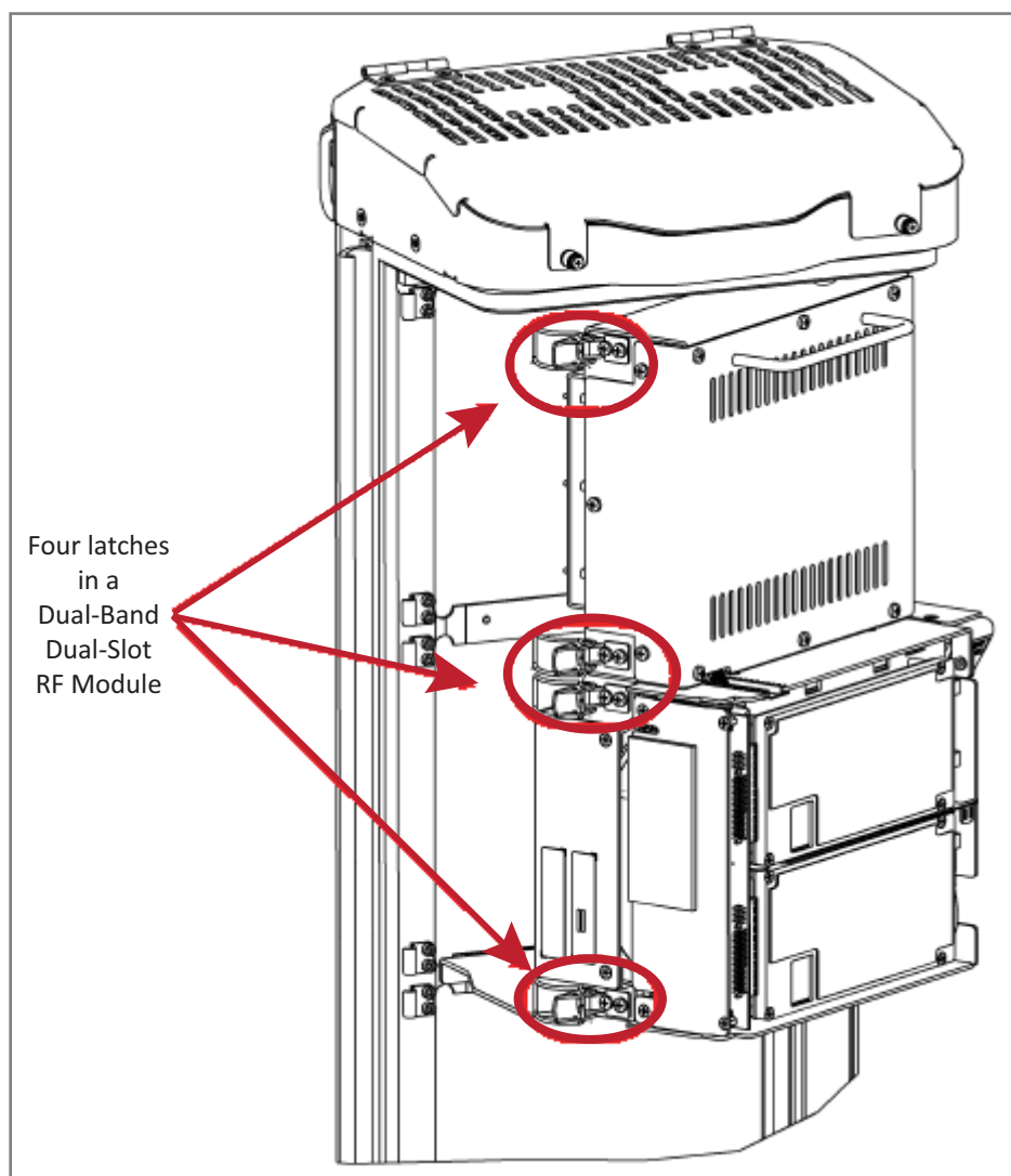
Figure 29. Dual-Bay RF Module Latches
