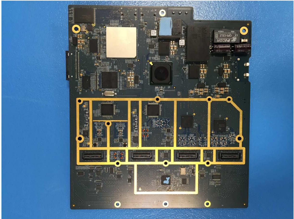
Motherboard - Back
