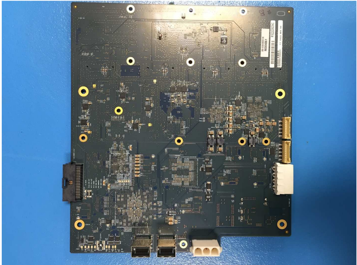
Motherboard - Front
