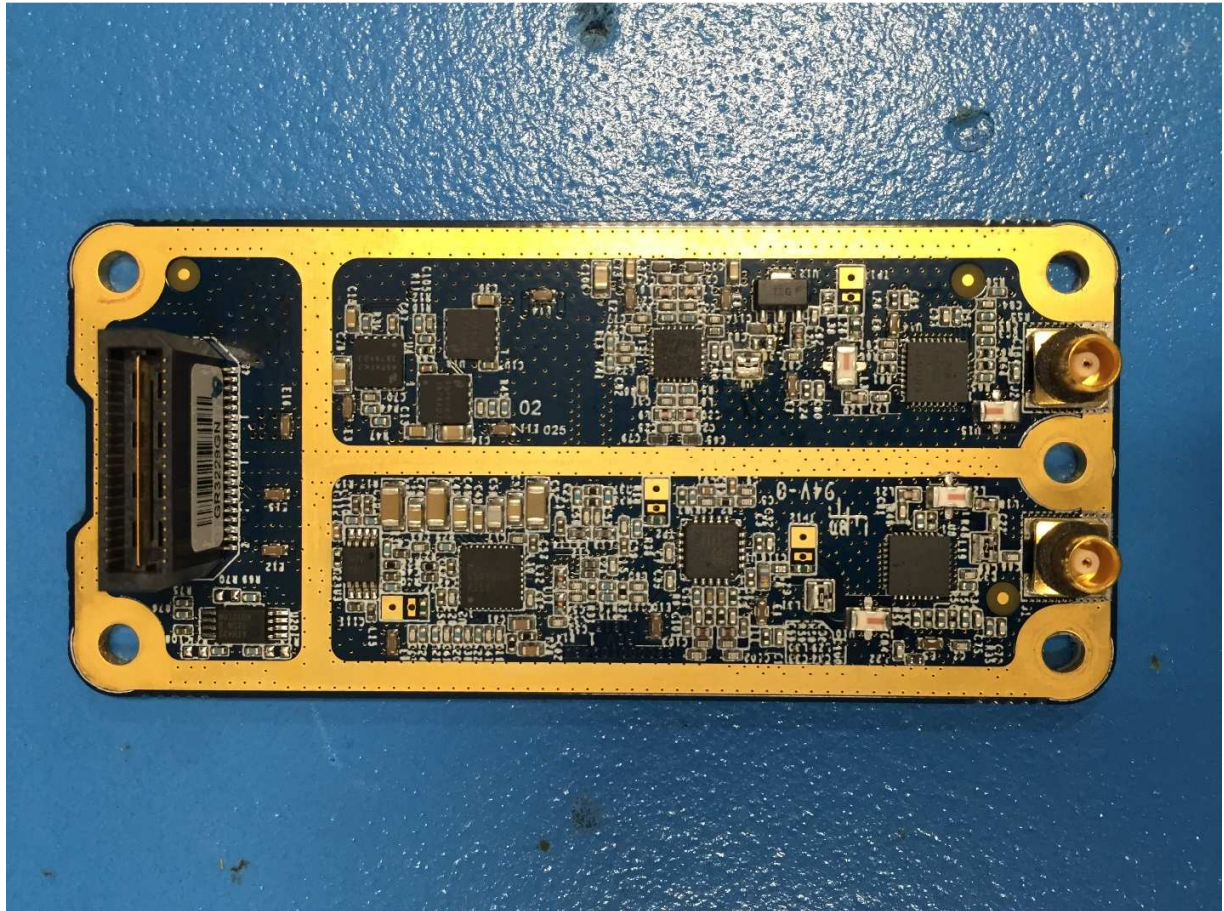
TX Card – Front
