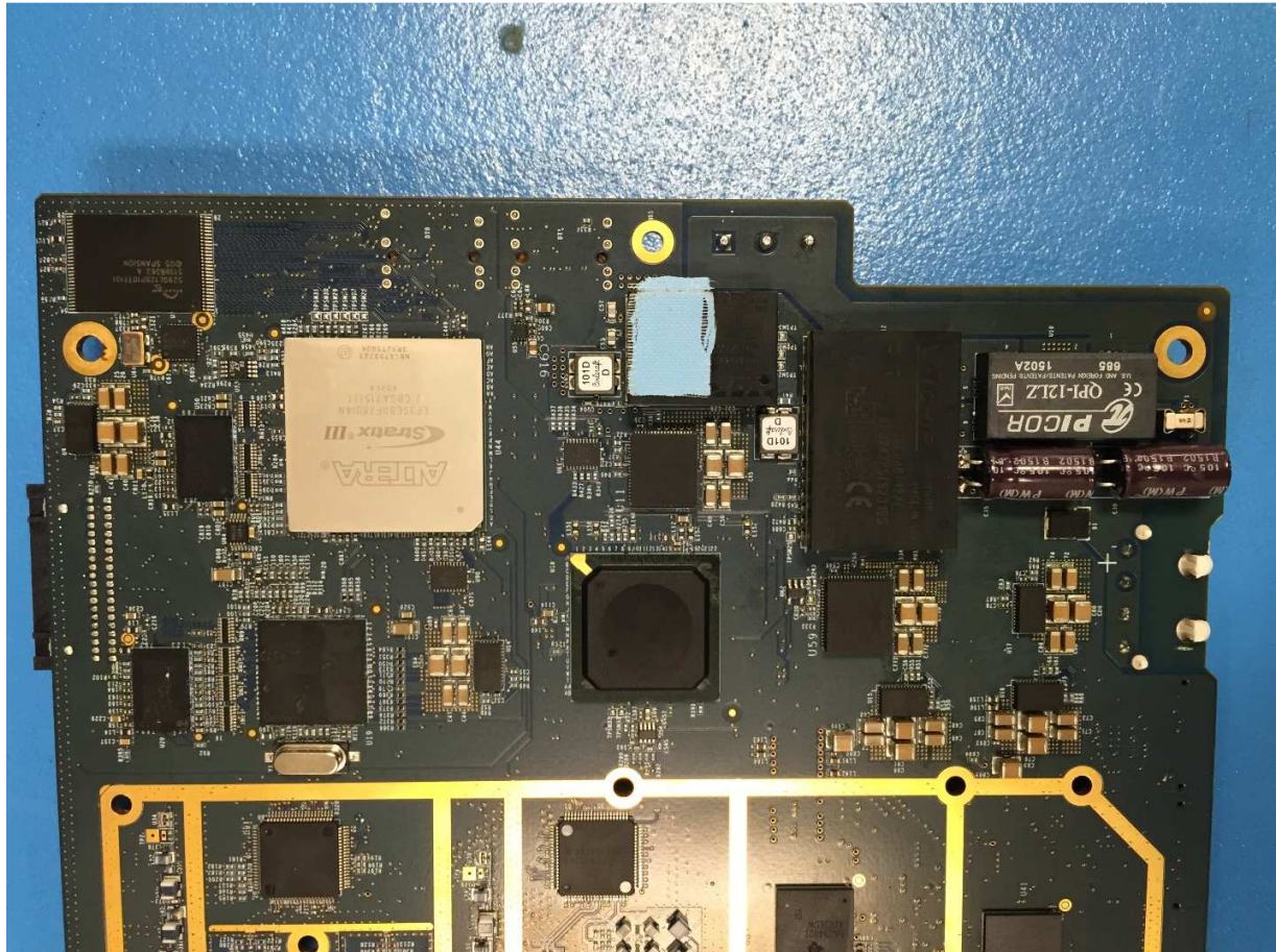
Motherboard – Back #3
