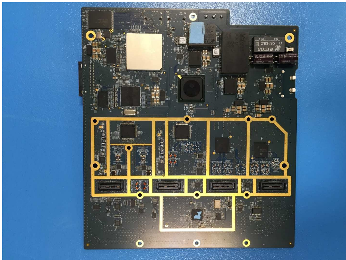
Motherboard - Back
