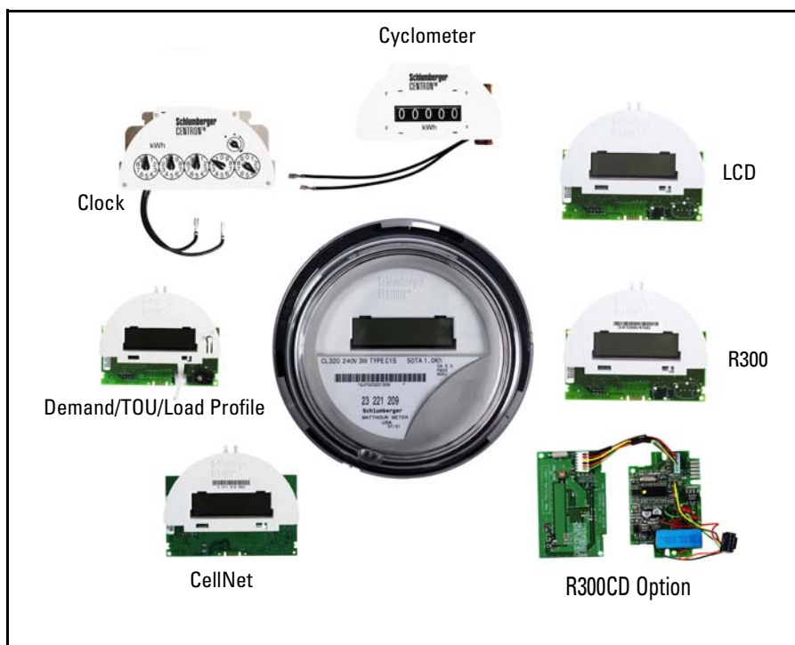
Figure 1.1 Personality Modules
