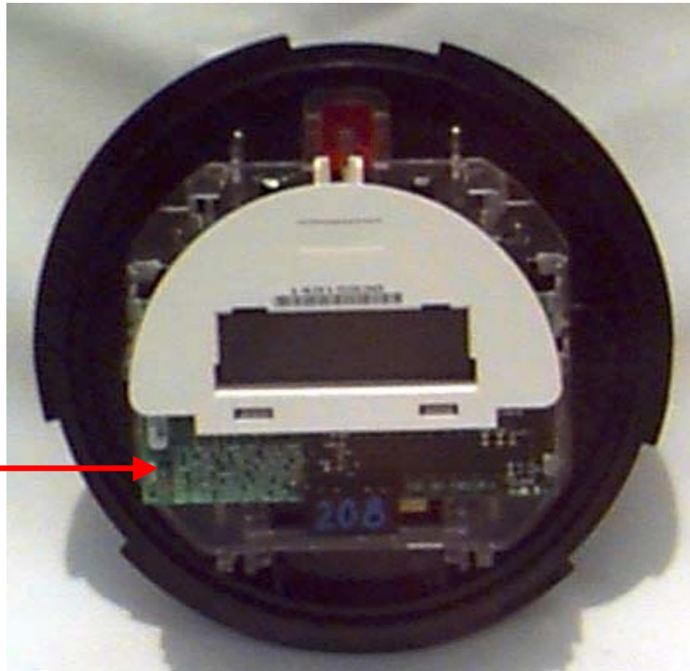
(c) Centron RMR Meter - Glass and Plastic Cover Removed
