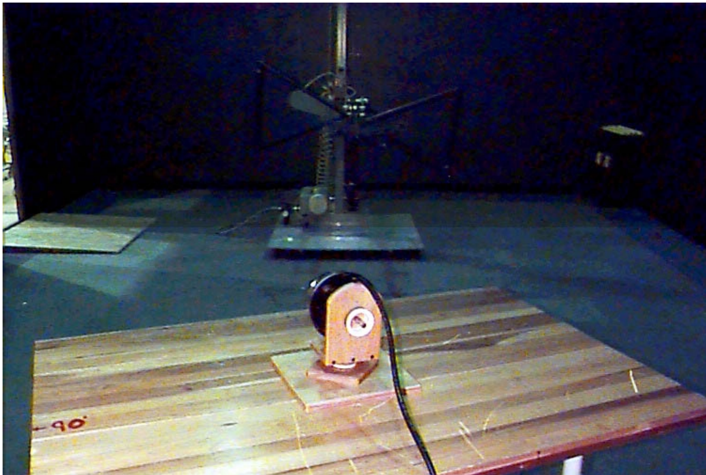
Radiated Emissions Test Setup - Rear View
