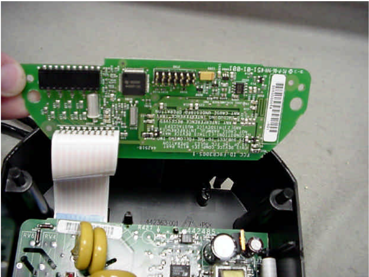
Photo 11. EUT, Top View of Transmitter Board
