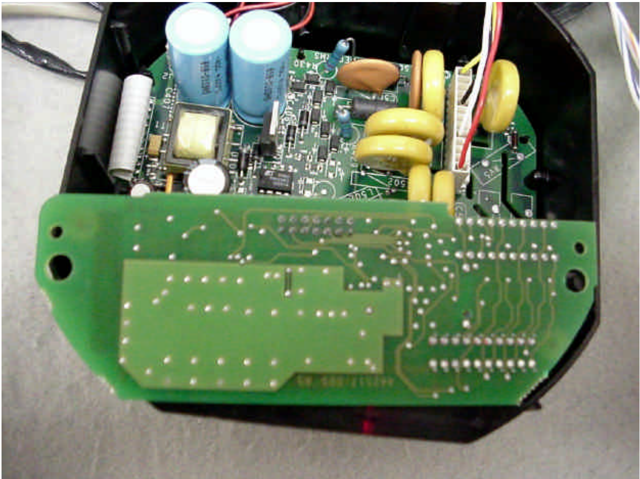
Photo 12. EUT, Bottom View of Transmitter Board
