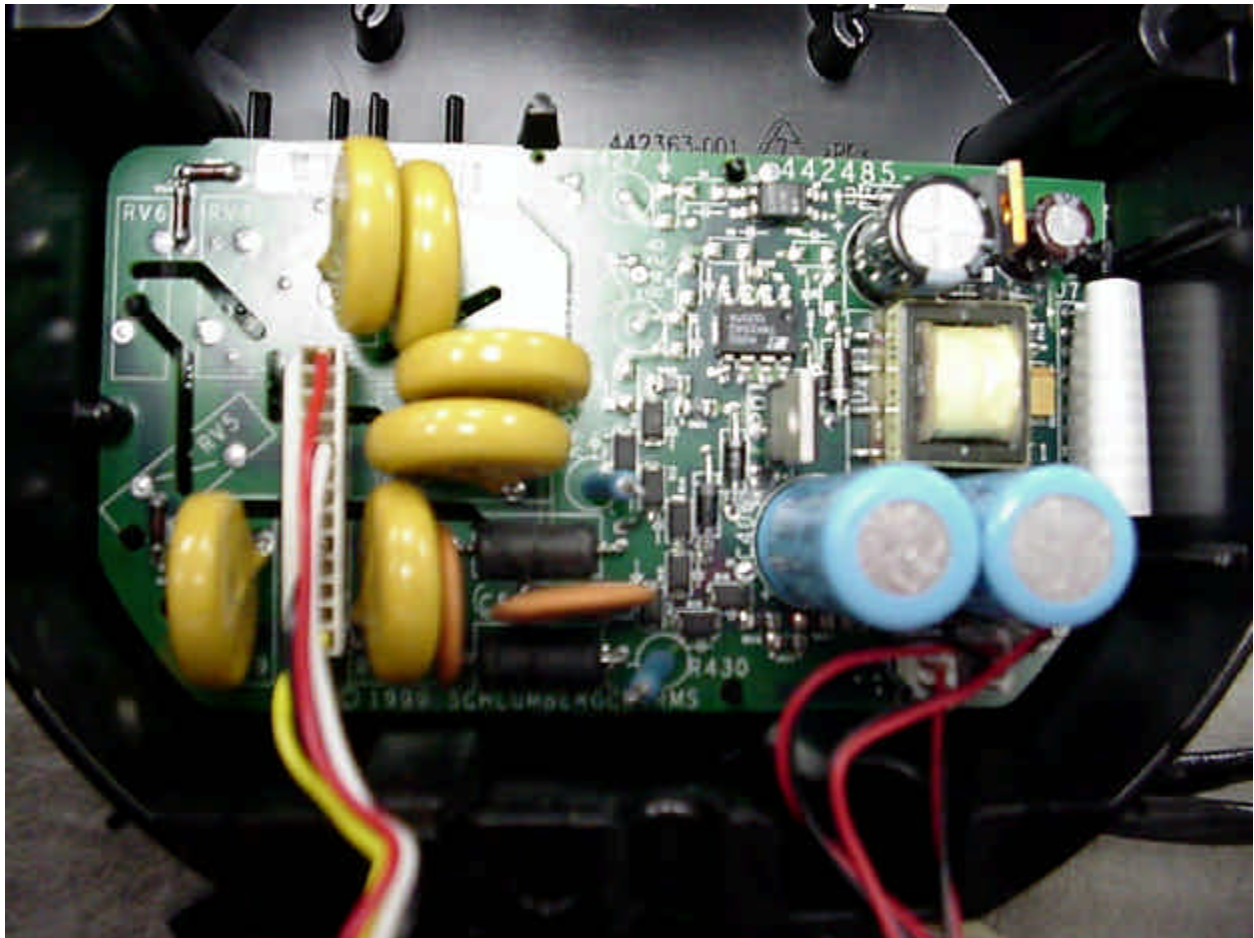
Photo 9. EUT, Top View of Power Supply Board
