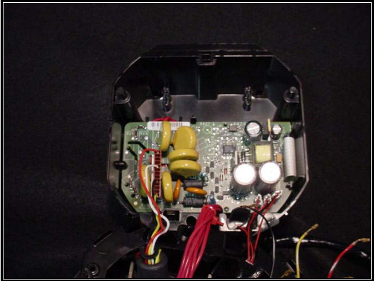
Figure B3: Face Plate and RF Board Removed Exposing Top Side of Power Supply Board
