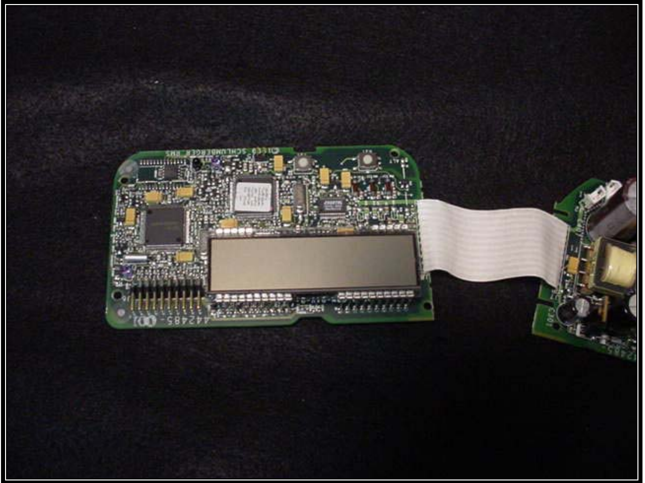
Figure B9: Top Side of Display Board
