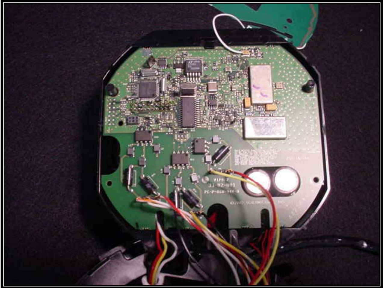
Figure B2: Face Plate Removed Exposing Topside of RF Board
