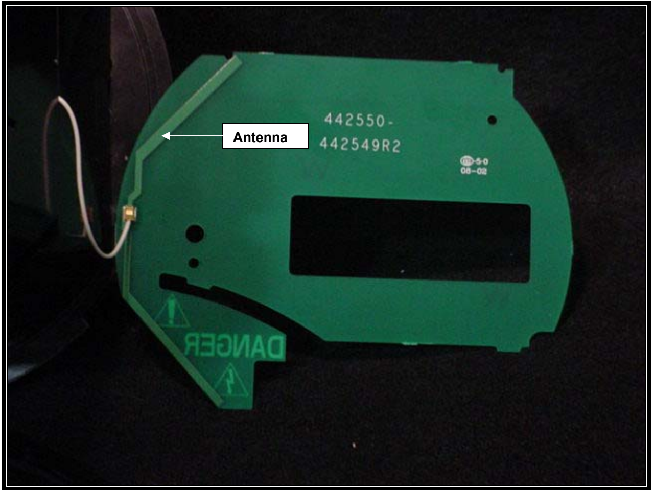
Figure B4: Back Side of Face Plate with Antenna
