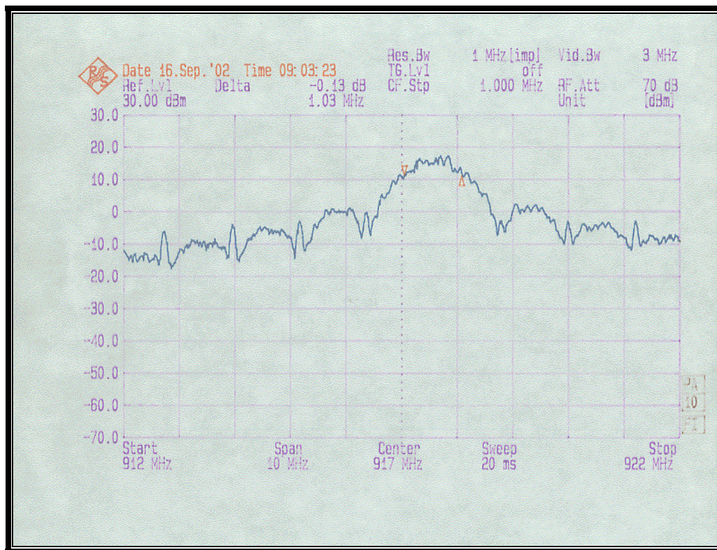
Figure 7.5-1: 6dB Bandwidth
