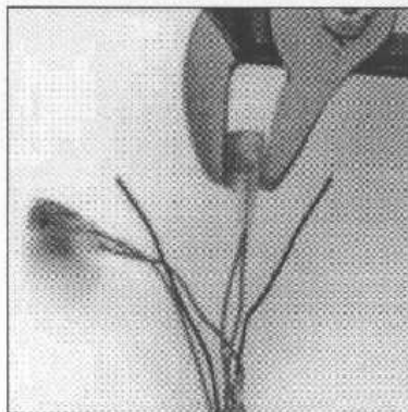
Figure 2-9. Depressing the Scotchlok Button
