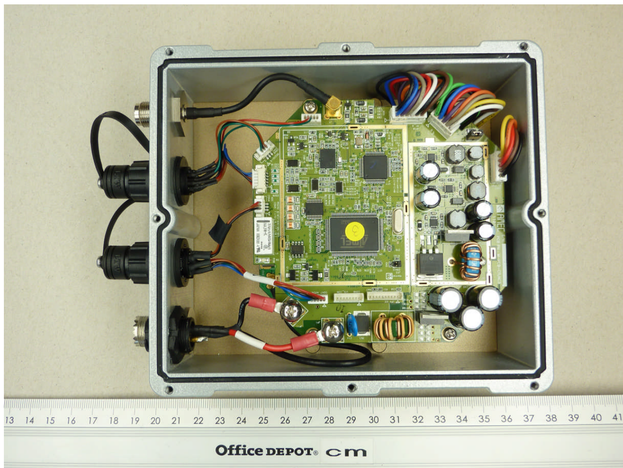
110939eut1.jpg: EUT, internal-view
