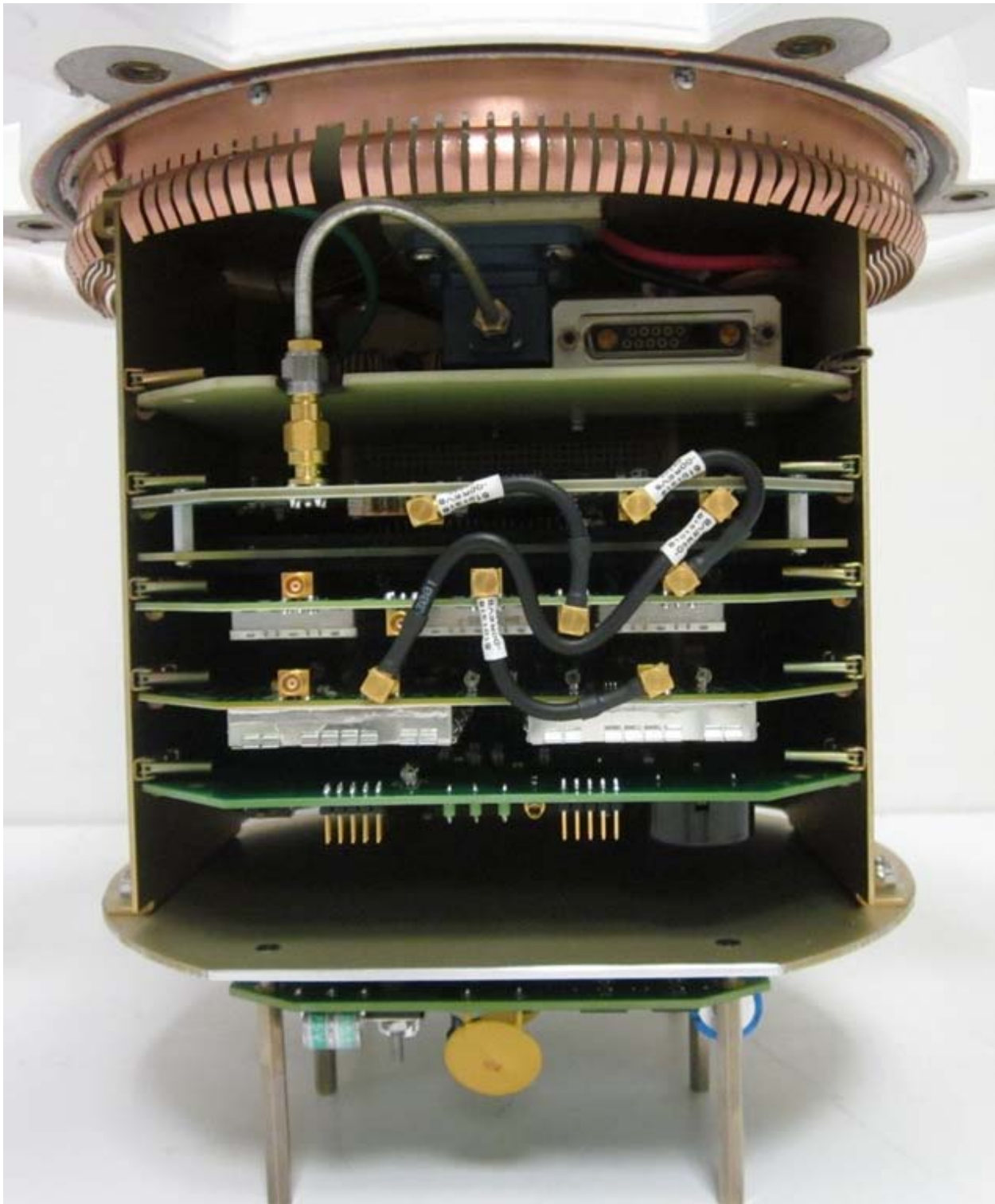
Lower Assembly Uncovered, Board Stack Up Visible
