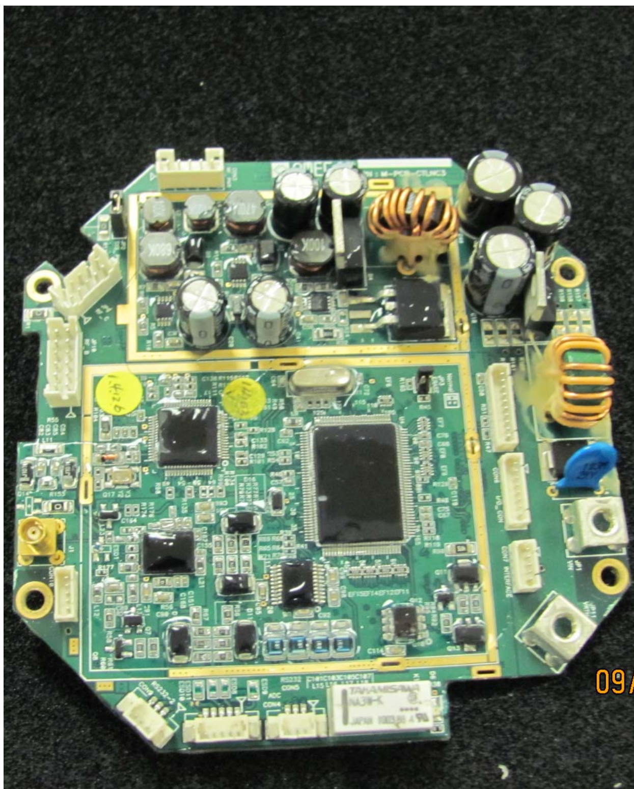
AIS Board 2
