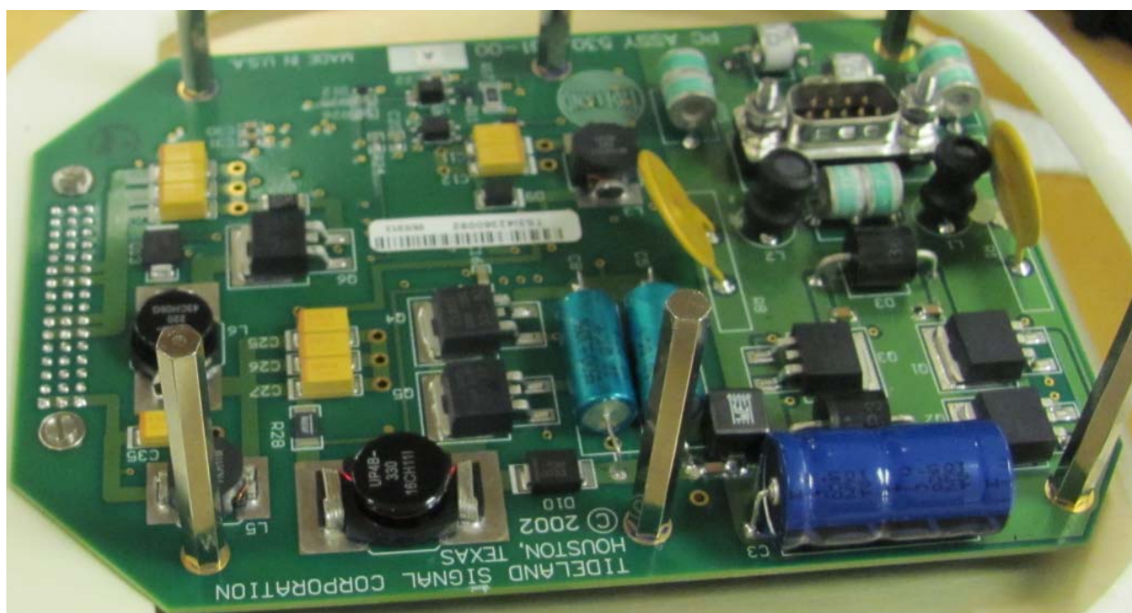
Power Supply Module
