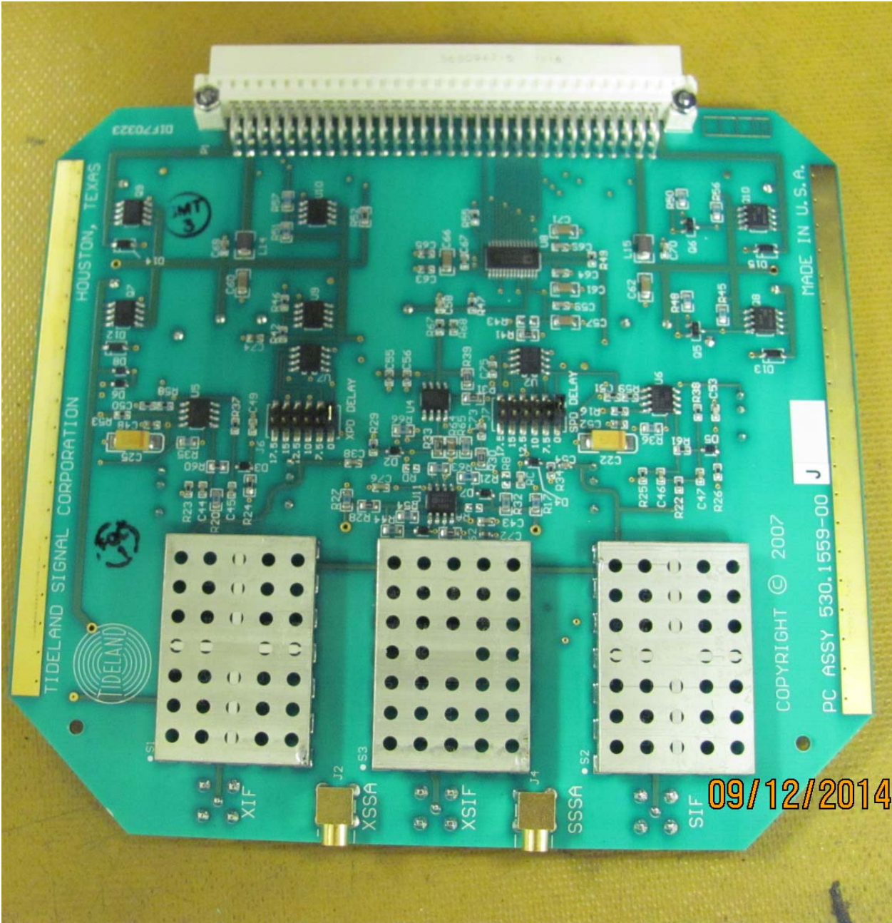
Dual Interface Module
