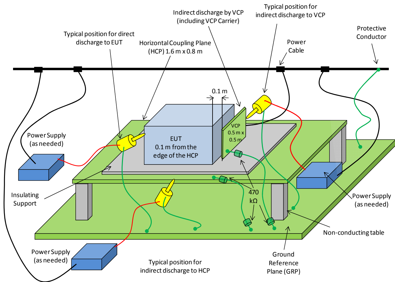
Figure 4.2.1.1: Electrostatic Discharge Immunity Test Setup
