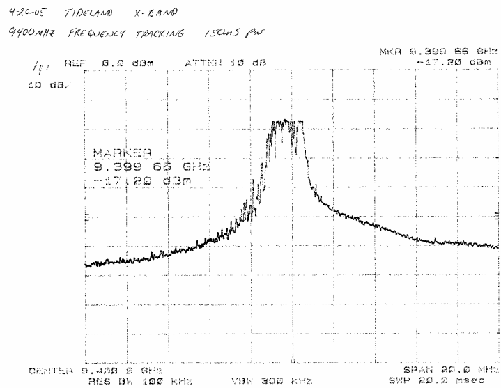
Figure 4.6.10 Frequency Tracking Accuracy 9400MHZ 150nS
