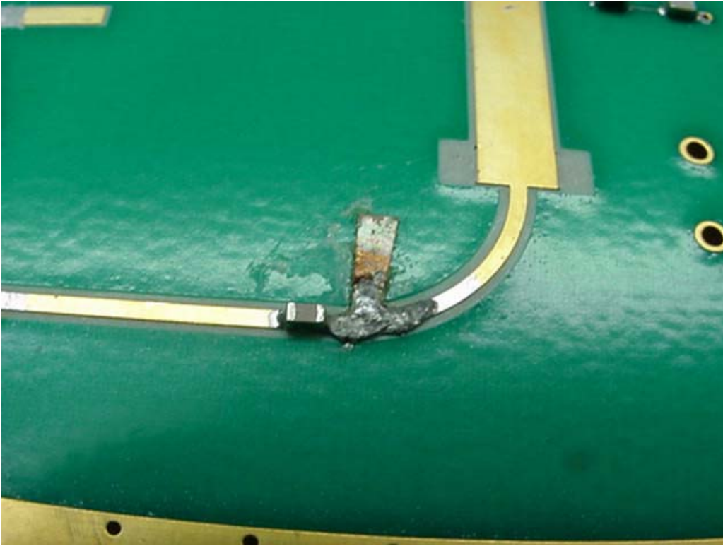
Photograph 4.22.2 SRF Cold Solder Joint
