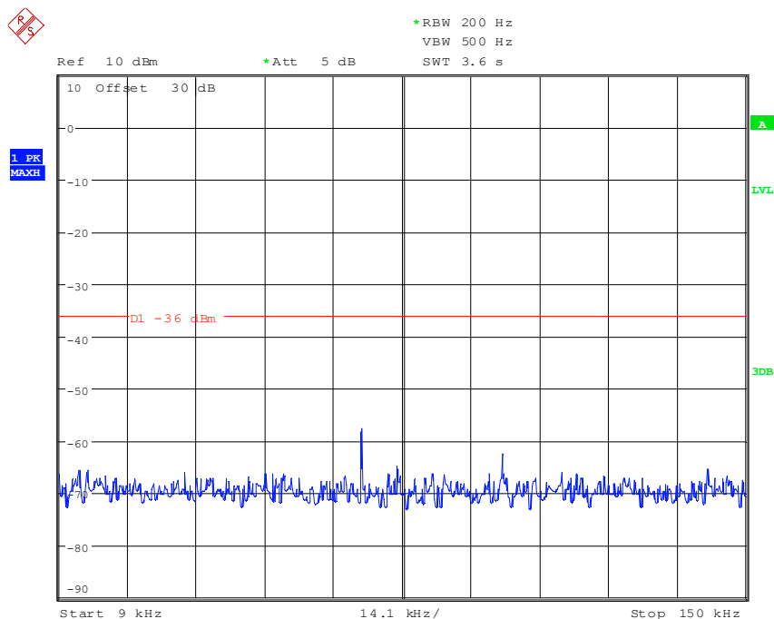
156TXH1.wmf: f = 9 kHz to 150 kHz, transmit high power
