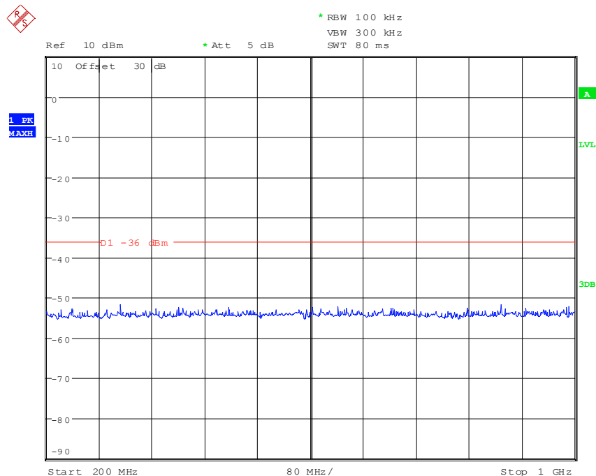
156TXL4.wmf: f = 200 MHz to 1000 MHz, transmit low power
