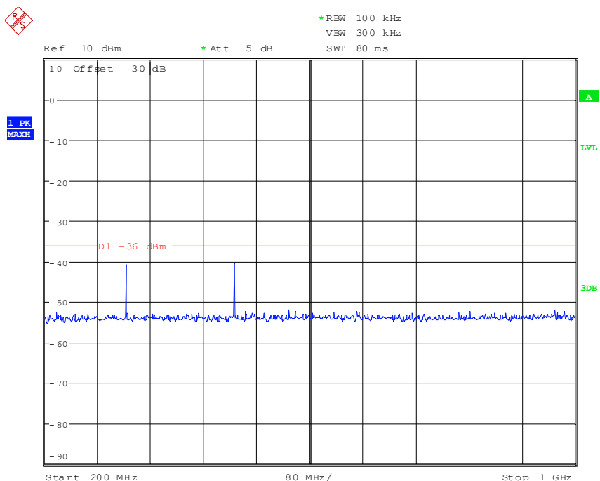
162TXH4.wmf: f = 200 MHz to 1000 MHz, transmit high power
