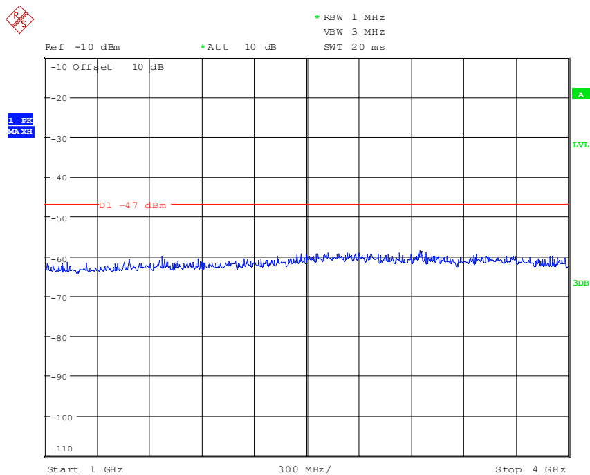
156RX5.wmf: f = 1 GHz to 4 GHz
