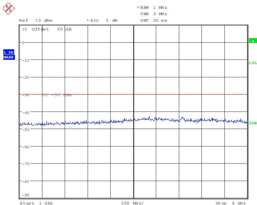
156TXH5.wmf: f = 1 GHz to 4 GHz, transmit high power
