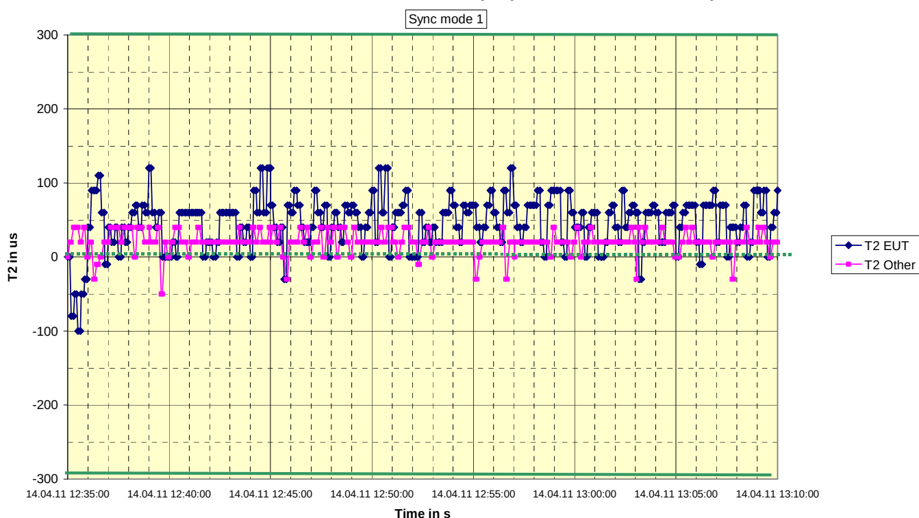
2011-04-14 Ba - AMEC AtoN Mando-303 - 8.2.1- Sync jitter deviation vs. time in sync mode 1
