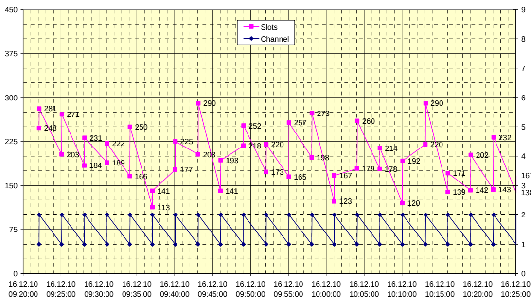
2010-12-16 AMEC Mando-303 - 8.1.8 Schedule mode B RATDMA message 6
