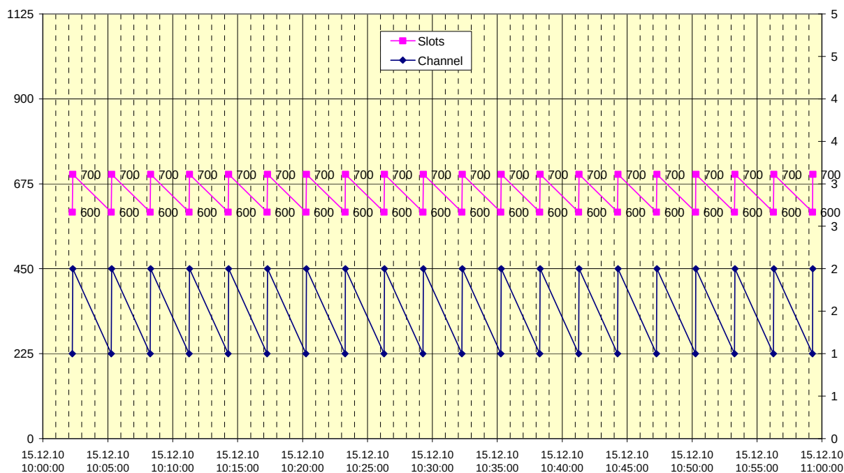
2010-12-15 AMEC Mando-303 - 8.1.8 Schedule FATDMA mode C message 6
