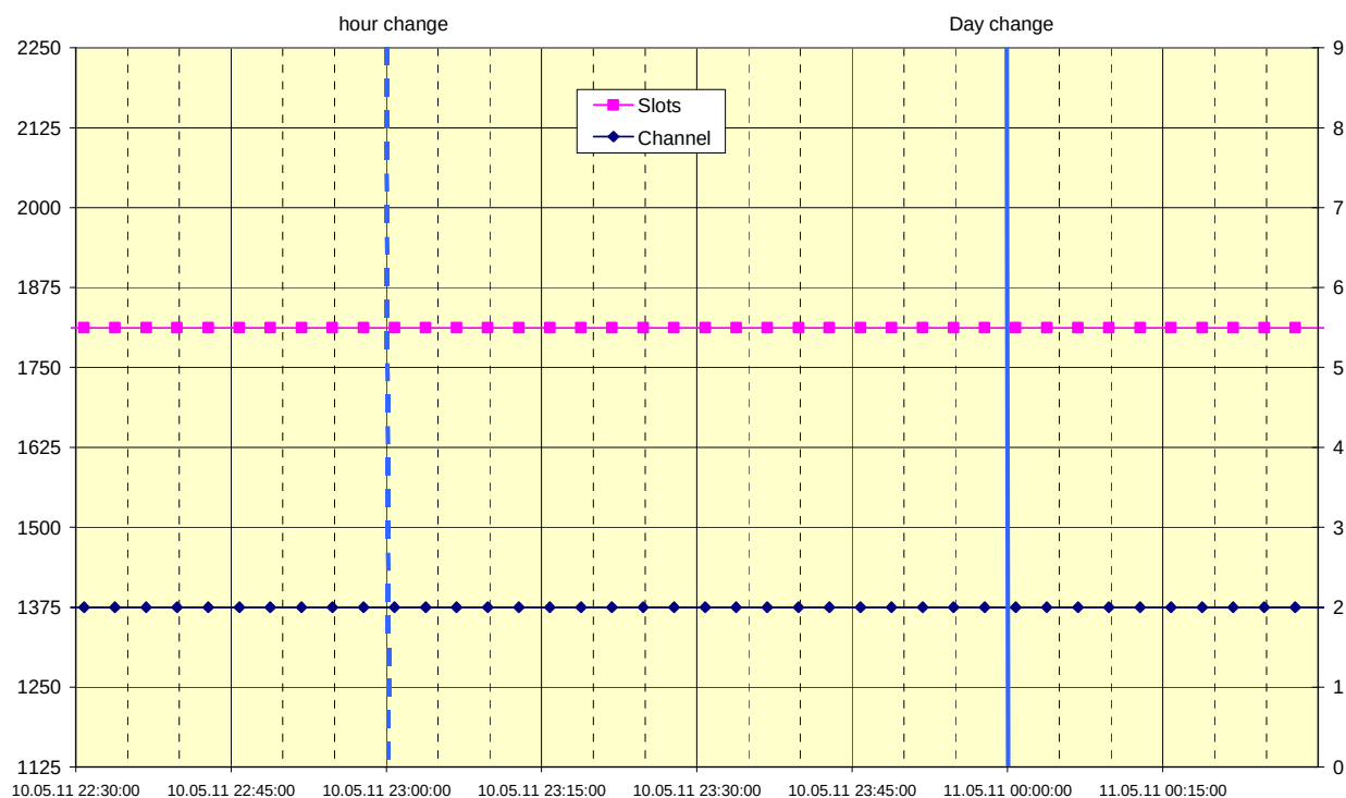
2011-05-11 Ba - AMEC Mando-301 - 8.1.4 Schedule mode C FATDMA message 21, Channel B
