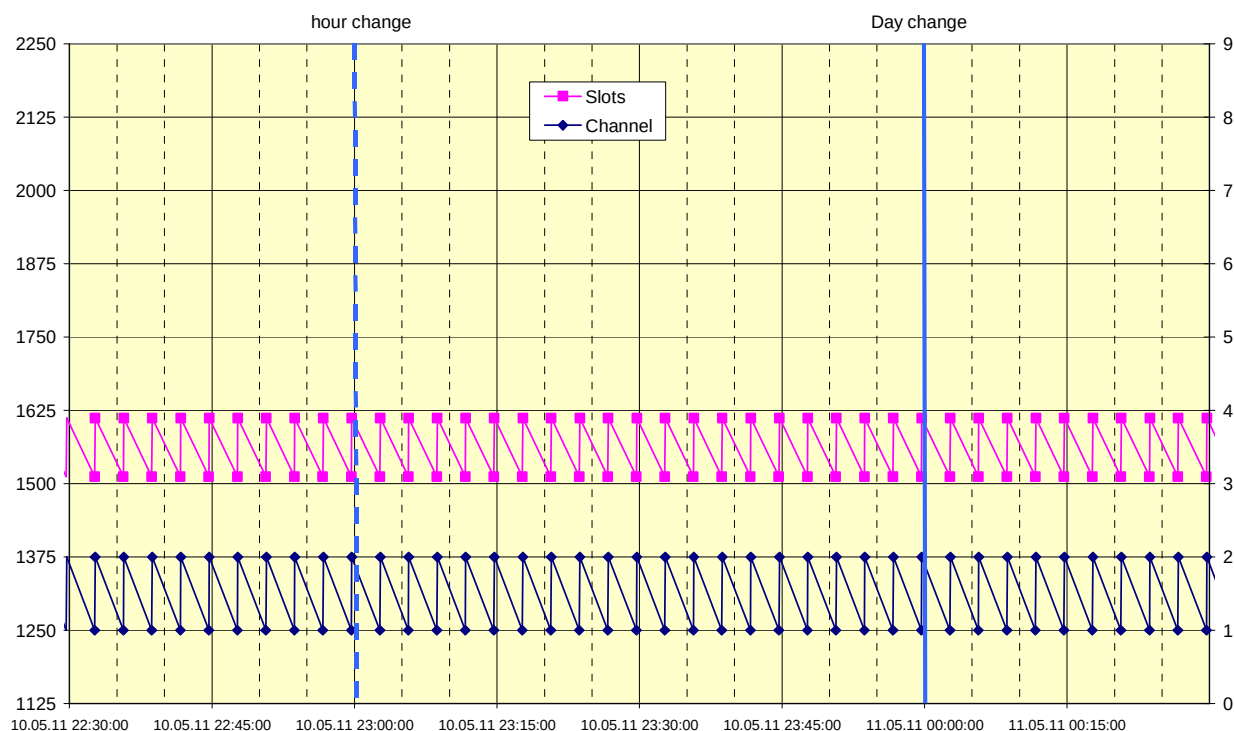
2011-05-11 Ba - AMEC Mando-301 - 8.1.3 Schedule mode B FATDMA message 21
