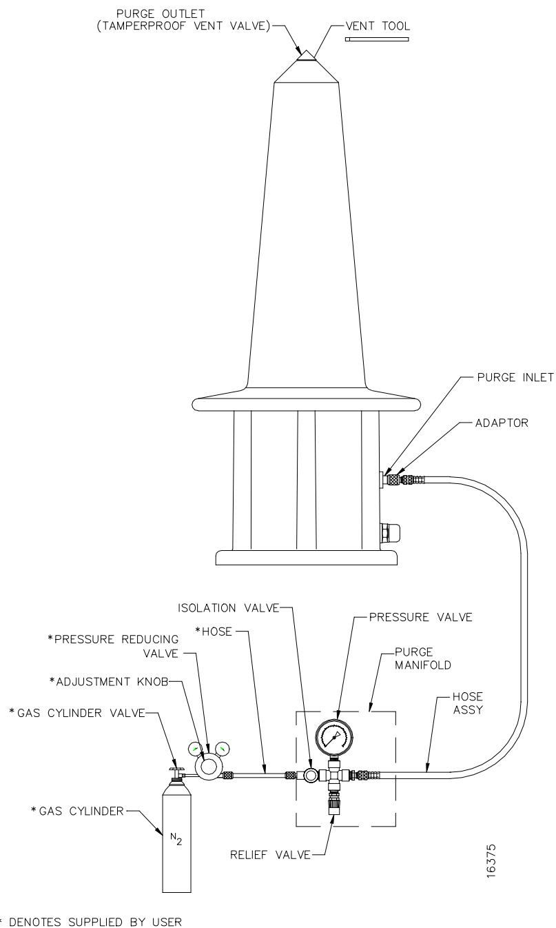
Figure 3.1 Racon Purging Operation
