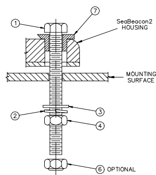
STANDARD MOUNTING HARDWARE DETAIL (3 OR 4 PLACES)
