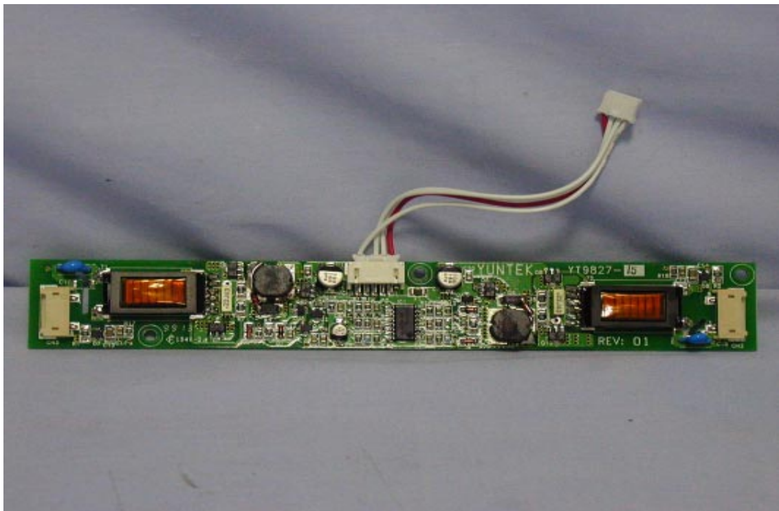
Main Board Component Side View of Inverter
