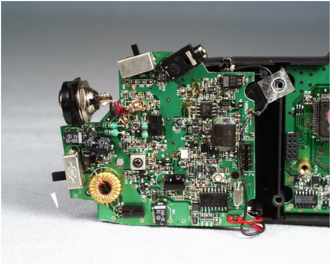
Side B of the Venture-Express (Main board)
