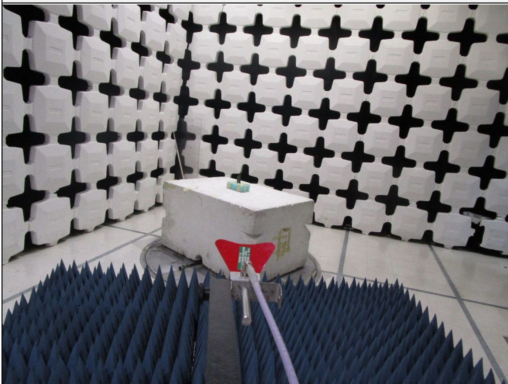
Test Setup for Radiated Emissions: 1 – 2GHz, Vertical Polarization
