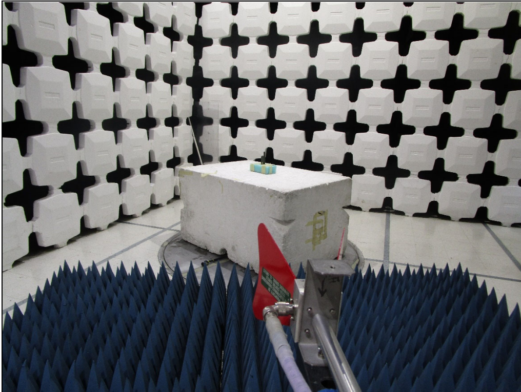
Test Setup for Radiated Emissions: 1 – 2GHz, Horizontal Polarization
