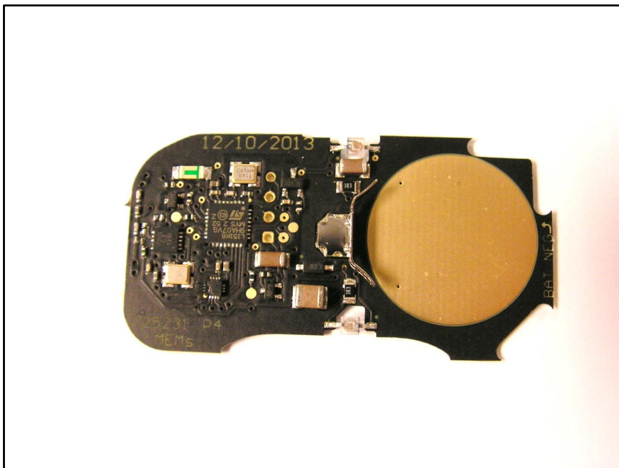
Top View
