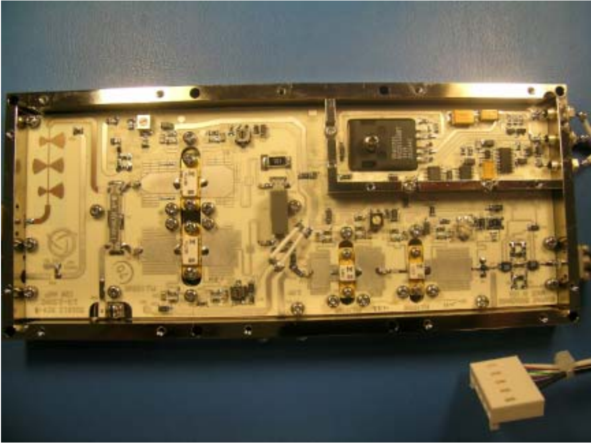
906816-1 Power Amplifier assy.
