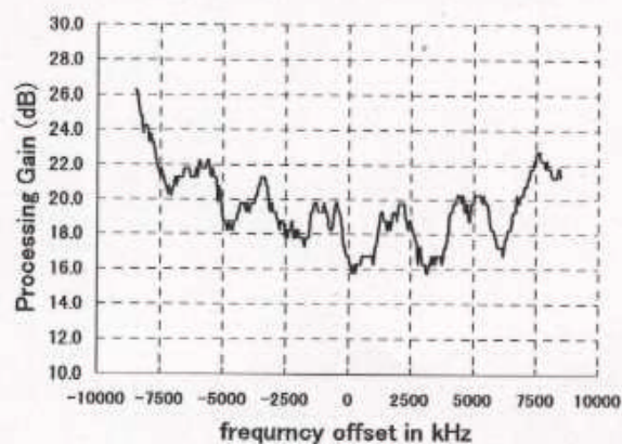
Processing gain at channel 9 with CW
