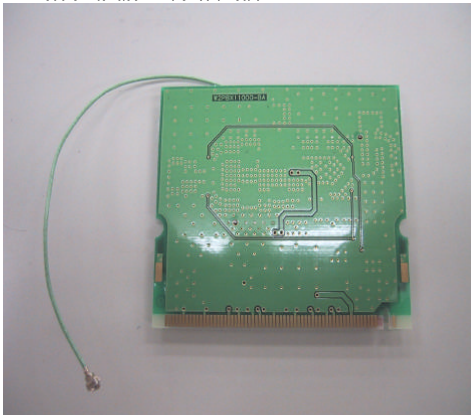
Back View of RF Module Interface Print Circuit Board
