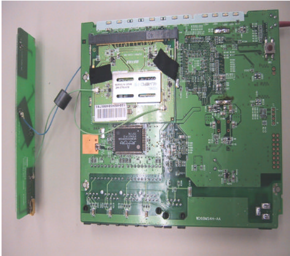
Back View of Print Circuit Board Put Off Enclosure
