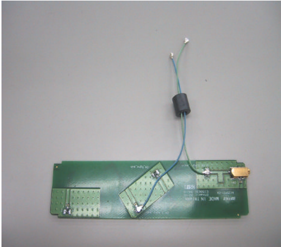
Back View of Antenna Print Board
