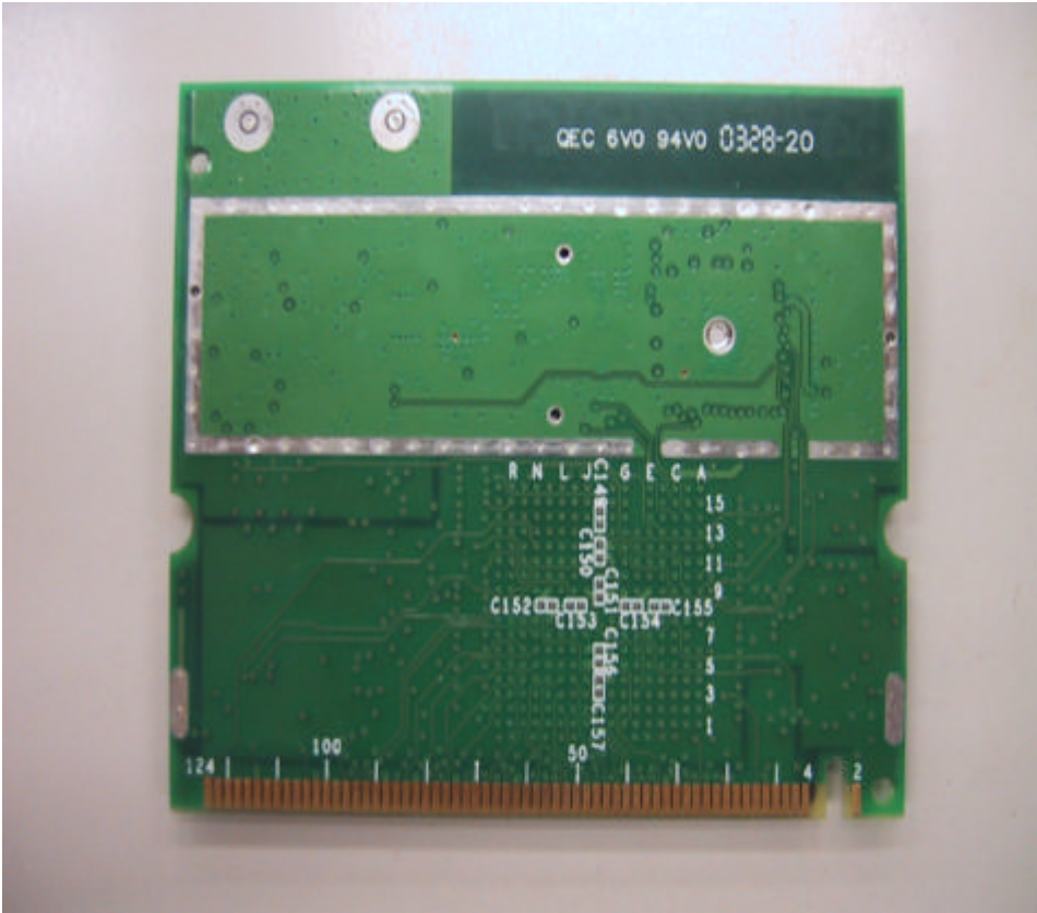
Back View of RF Module Print Circuit Board
