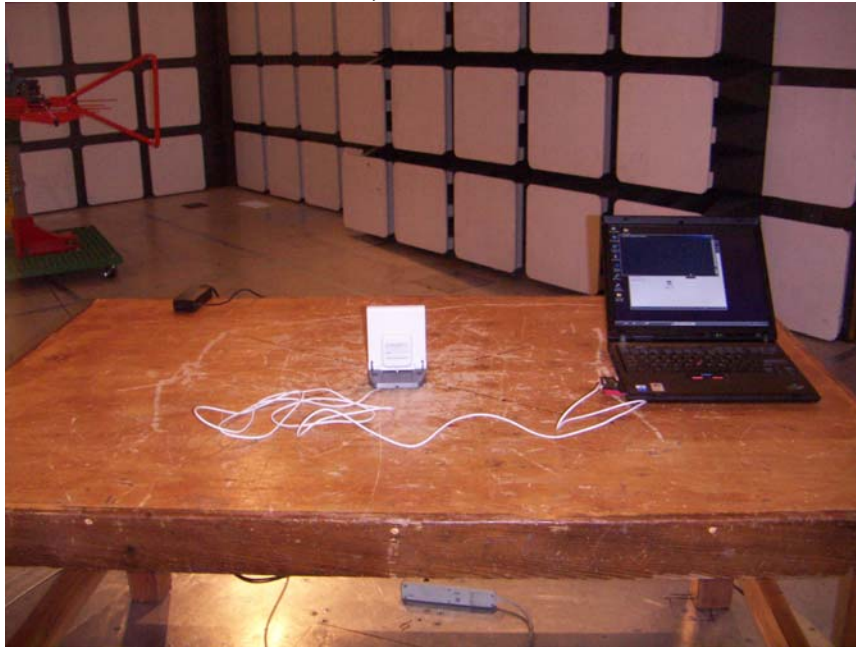
RADIATED FRONT PHOTO , WLE-DA ANTENNA
