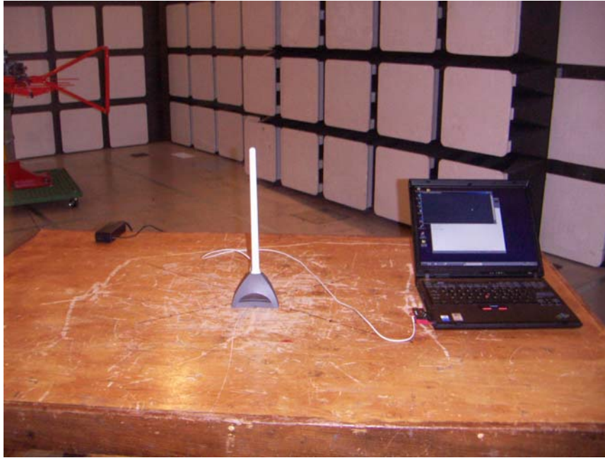
RADIATED FRONT PHOTO , WLE-HG-NDR ANTENNA
