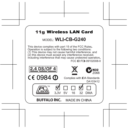
Size:40x40 R2.5
