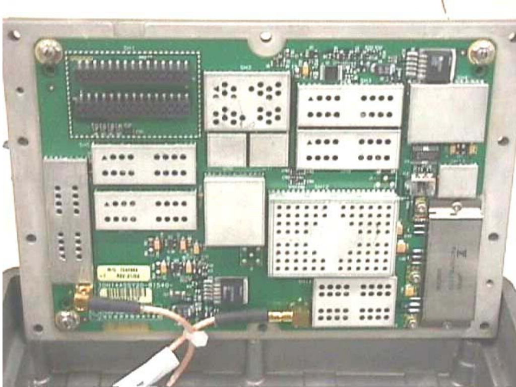
RF BOARD
