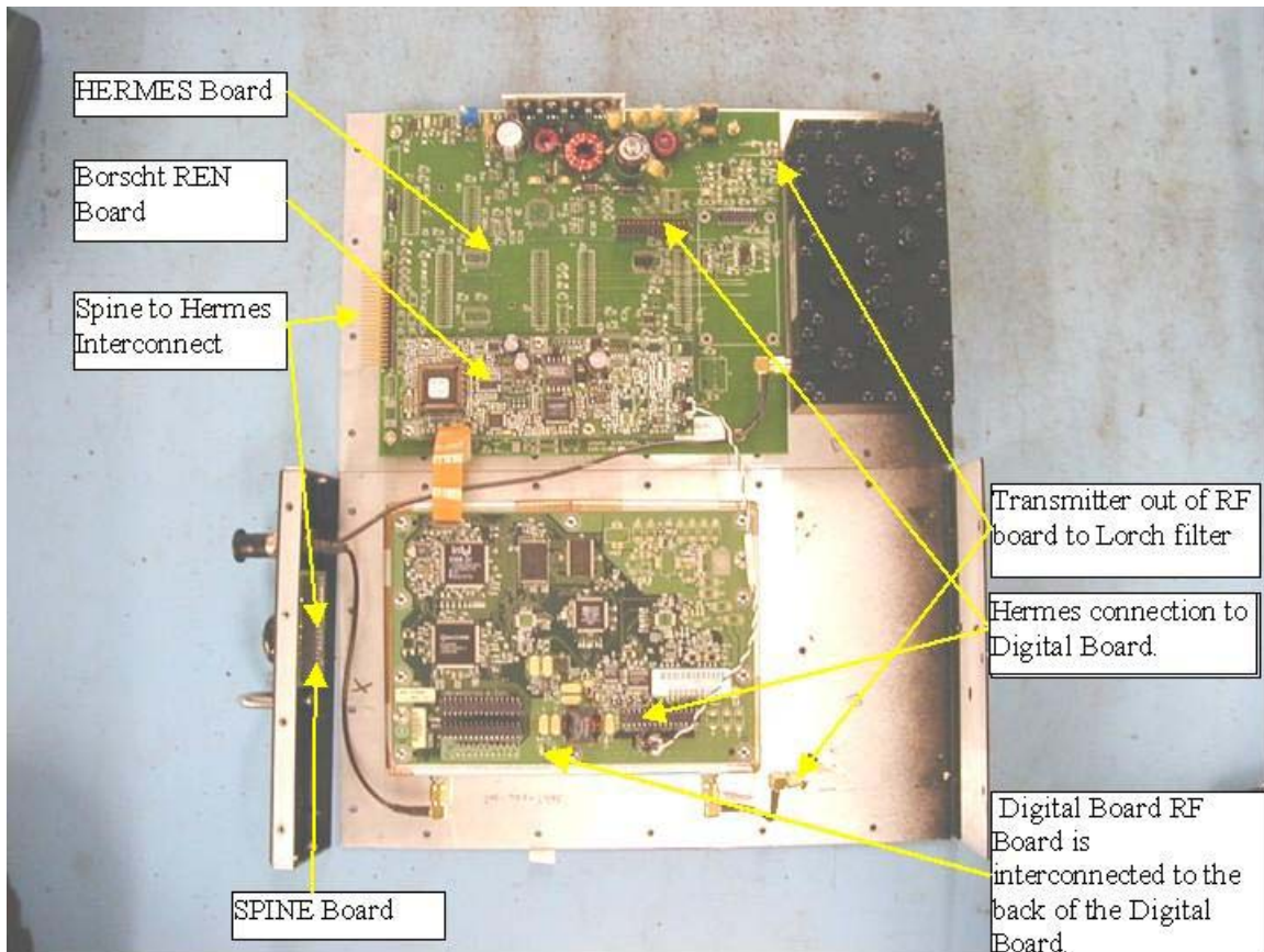
RCOM-100 OPENED AND LABELED
