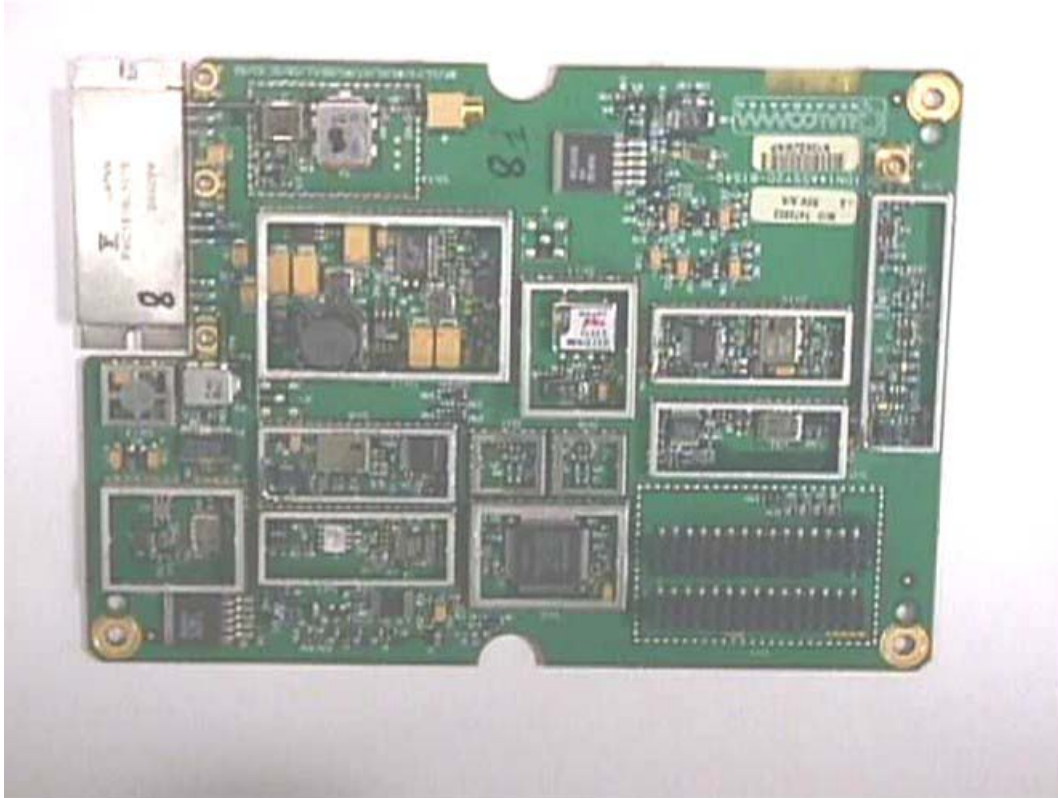
RF BOARD WITH SHIELDS REMOVED
