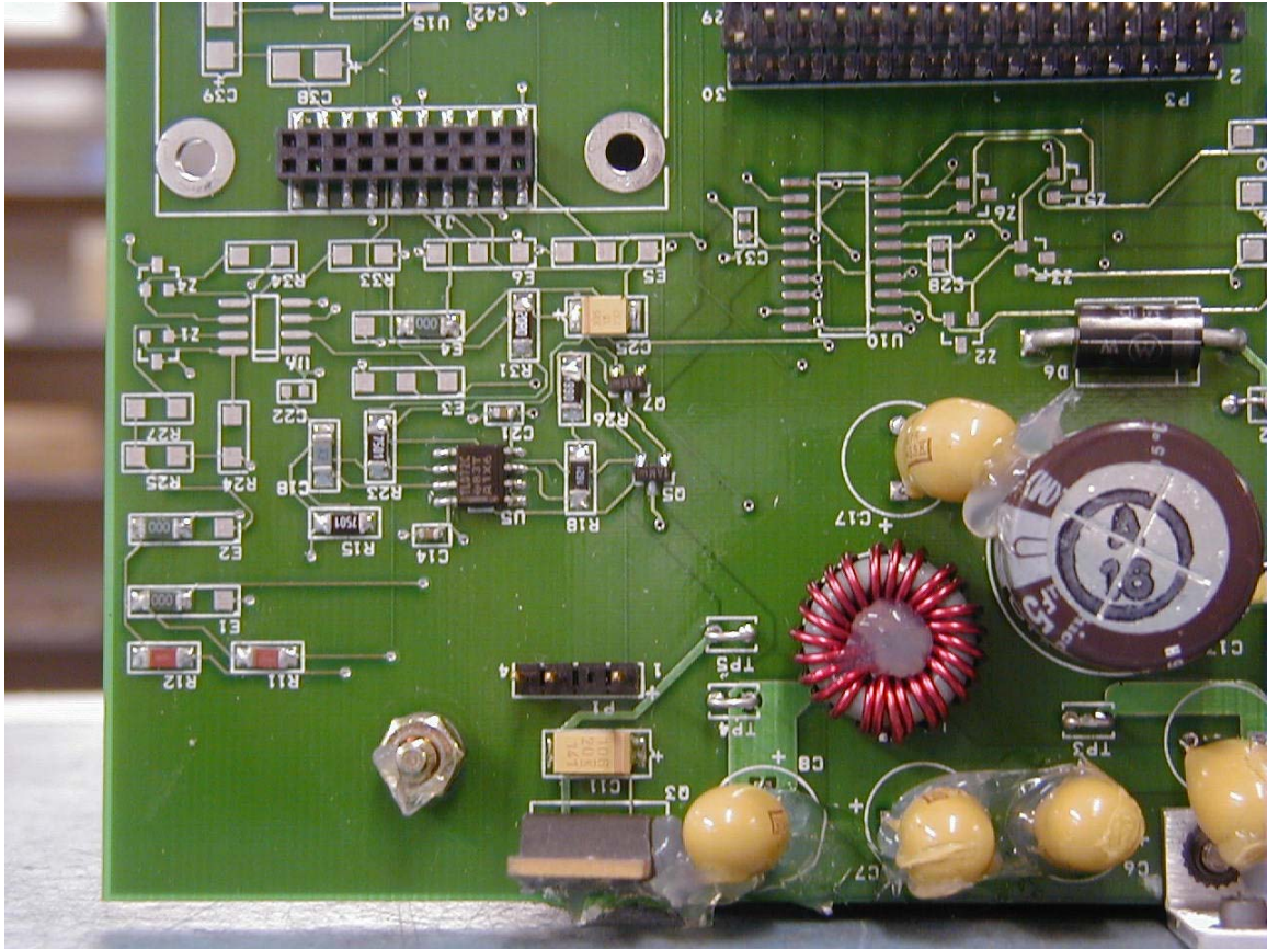
HERMES BOARD ZOOM
