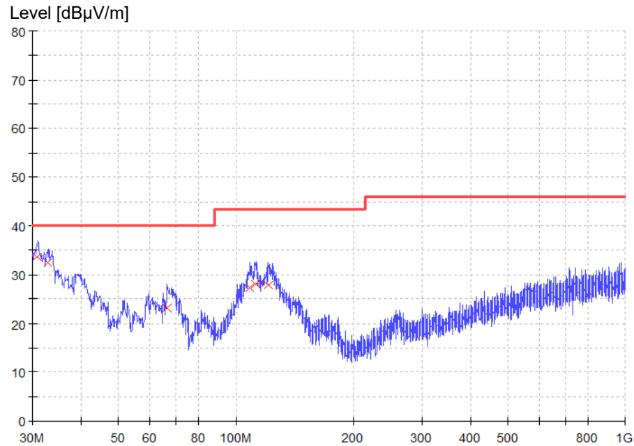
Figure 3: Spectral Diagrams, Radiated Emission, 30 MHz – 1000 MHz, Vertical polarization
