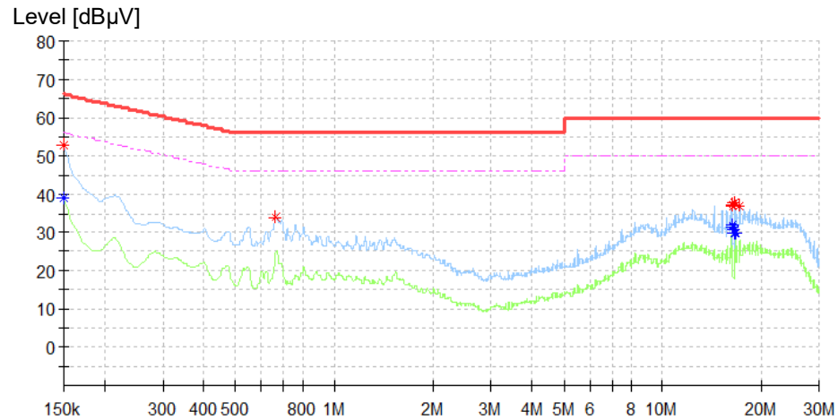
Figure 1: Spectral Diagrams, Conducted Emission, 150 kHz – 30 MHz, L&N
