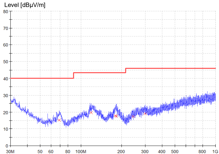
Figure 2: Spectral Diagrams, Radiated Emission, 30 MHz – 1000 MHz, Horizontal polarization
