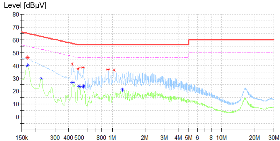
Figure 1: Spectral Diagrams, Conducted Emission, 150 kHz – 30 MHz, L Line
