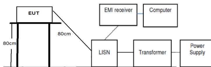
(Conducted emission)
