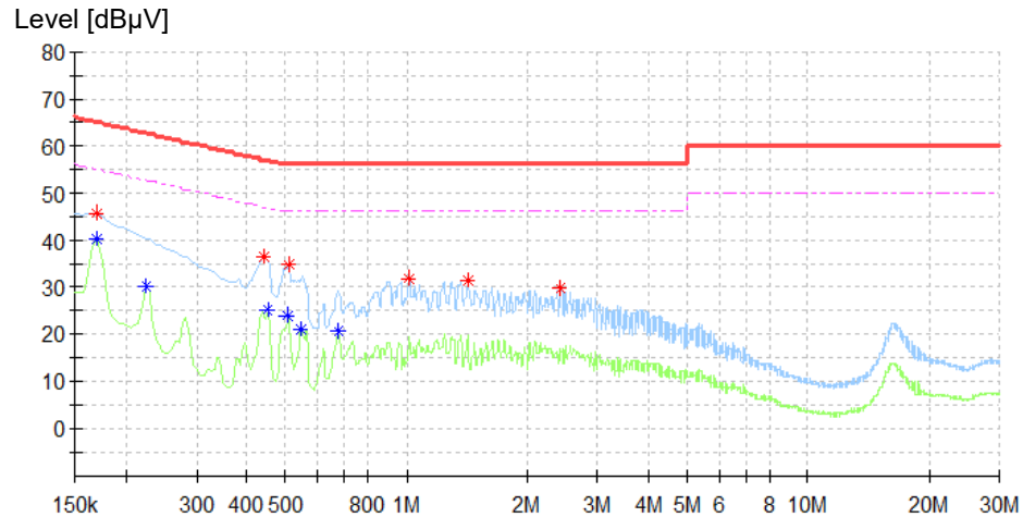
Figure 2: Spectral Diagrams, Conducted Emission, 150 kHz – 30 MHz, N Line
