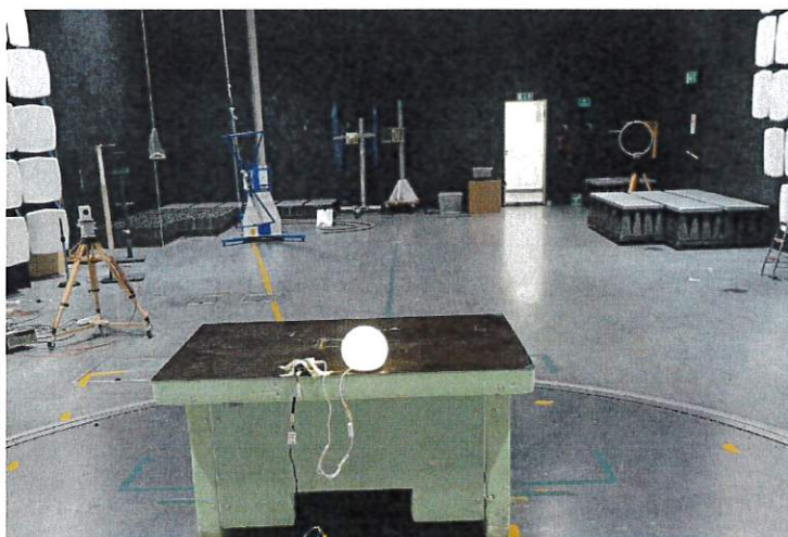
Test set up radiated emission 30 MHz – 1 GHz
