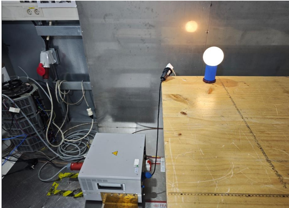
Photograph 1: Set-up for measurement of conducted emission
