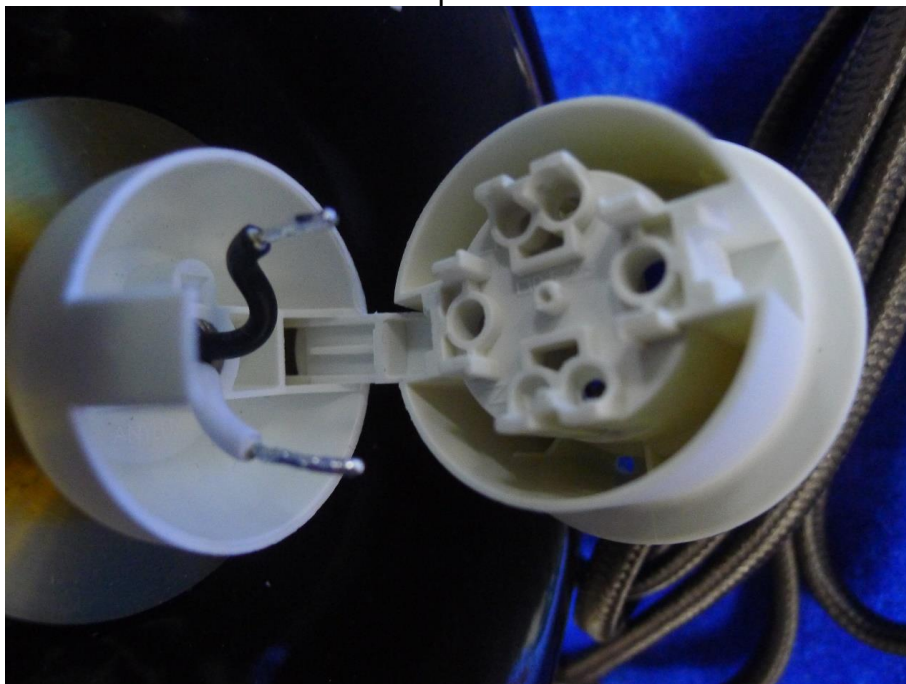
Internal View of Lampholder
