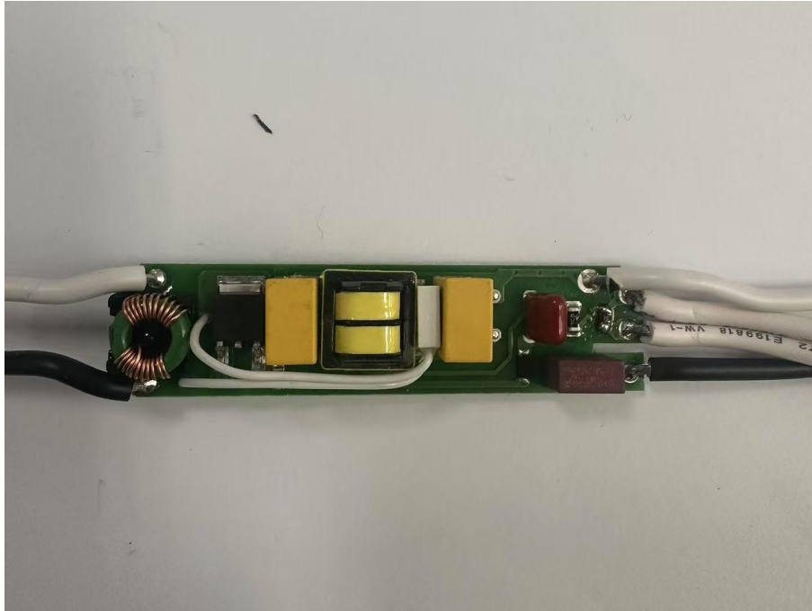
Dimmer PCB
