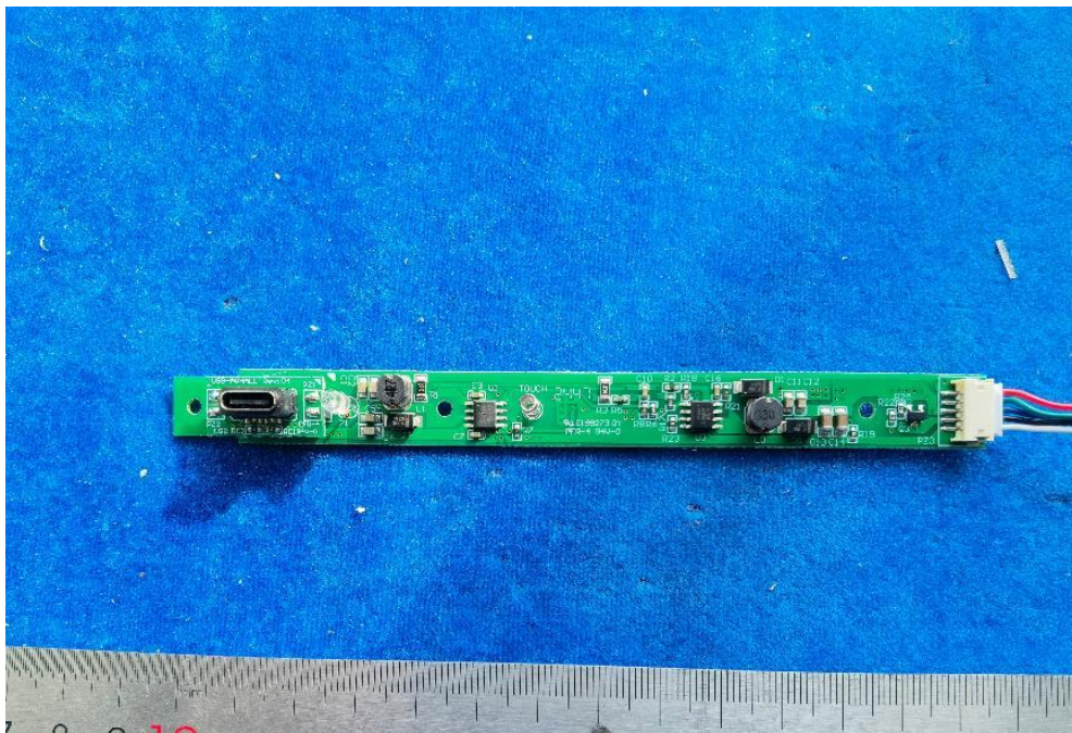
PCB of control module
