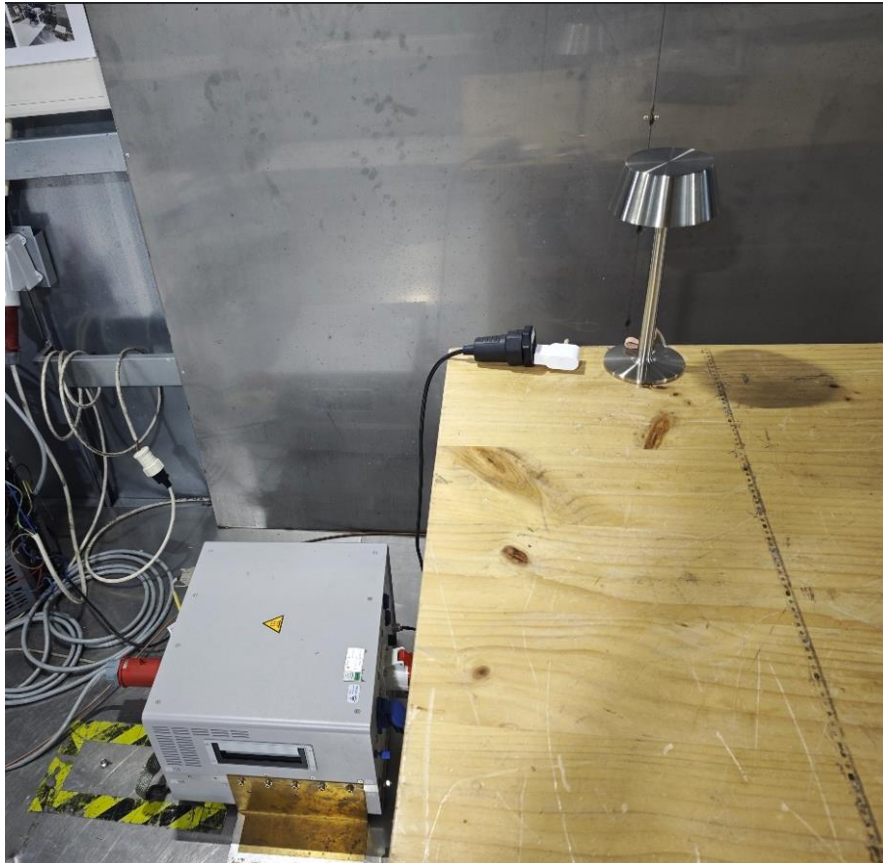
Photograph 1: Set-up for measurement of conducted emission
