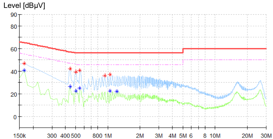
Figure 1: Spectral Diagrams, Conducted Emission, 150 kHz – 30 MHz, L
