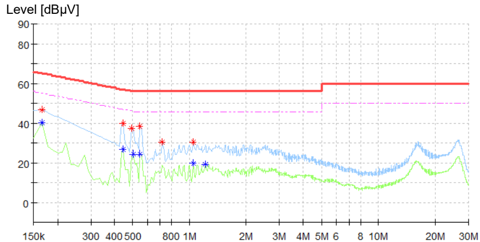
Figure 2: Spectral Diagrams, Conducted Emission, 150 kHz – 30 MHz, N
